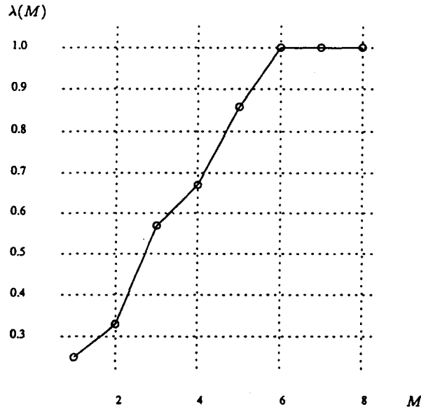
FIG. 10. Throughput \lambda(M) as a function of the number of customers M .
