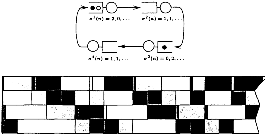
FIG. 9. CJN, four stations and three customers. Initial condition (Q^1, R^1) = (2, 2), (Q^2, R^2) = (0, 0), (Q^3, R^3) = (1, 0), (Q^4, R^4) = (0, 0) .
