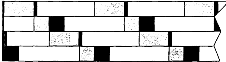
FIG. 7. (Q^1, R^1) = (1, 2), (Q^2, R^2) = (0, 0), (Q^3, R^3) = (1, 0), (Q^4, R^4) = (0, 0) .
