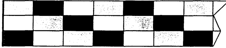
FIG. 5. Initial condition (Q^1, R^1) = (1, 1), (Q^2, R^2) = (0, 0), (Q^3, R^3) = (1, 1) .
