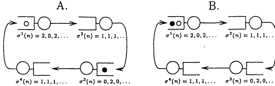
FIG. 6. CJN, four stations and two customers.
