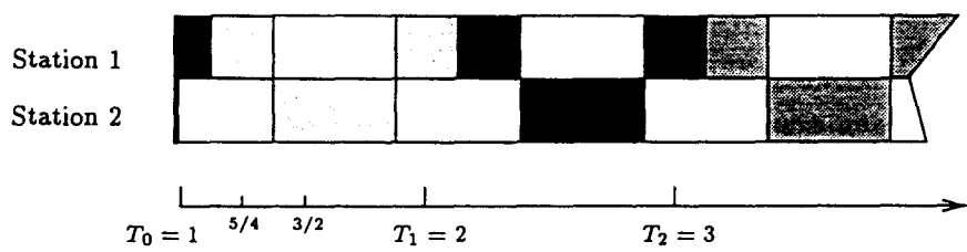
FIG. 2. Initial condition (Q^1, R^1) = (1, 9/8) , (Q^2, R^2) = (0, 0) .
