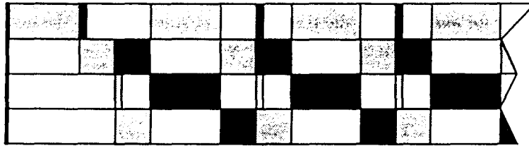
FIG. 8. (Q^1, R^1) = (2, 2), (Q^2, R^2) = (0, 0), (Q^3, R^3) = (0, 0), (Q^4, R^4) = (0, 0) .
