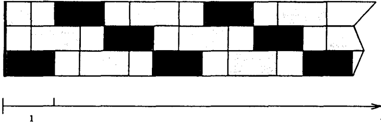
FIG. 4. Initial condition (Q^1, R^1) = (1, 1/2), (Q^2, R^2) = (0, 0), (Q^3, R^3) = (1, 1) .
