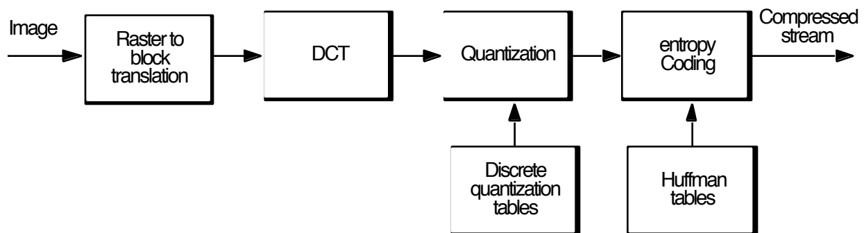
Figure 2. Simplified diagram of a discrete cosine transform (DCT) encoder. The processing steps are specified in the JPEG standard, while the tables are specified in each image.
