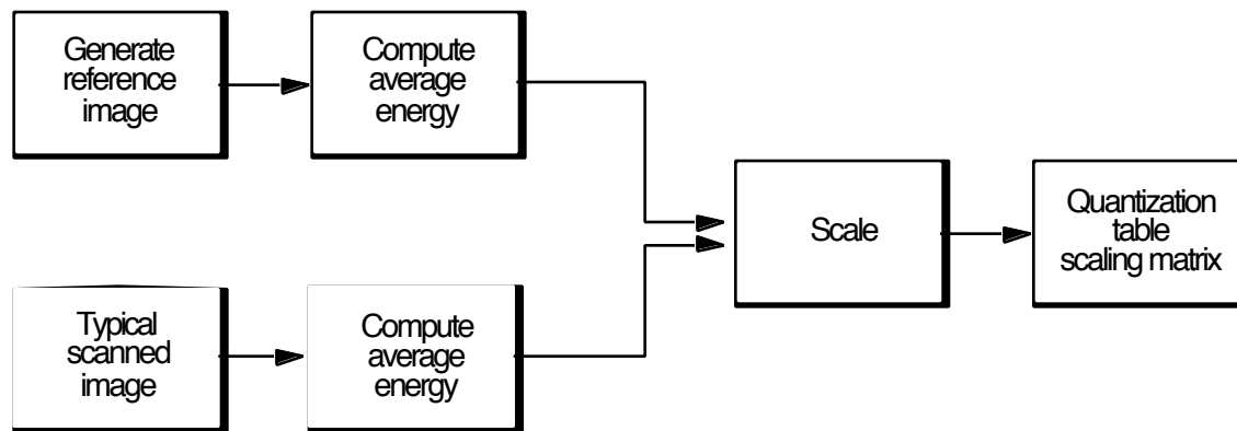
Figure 4. Sharpening an image in the JPEG domain during the encoding.
