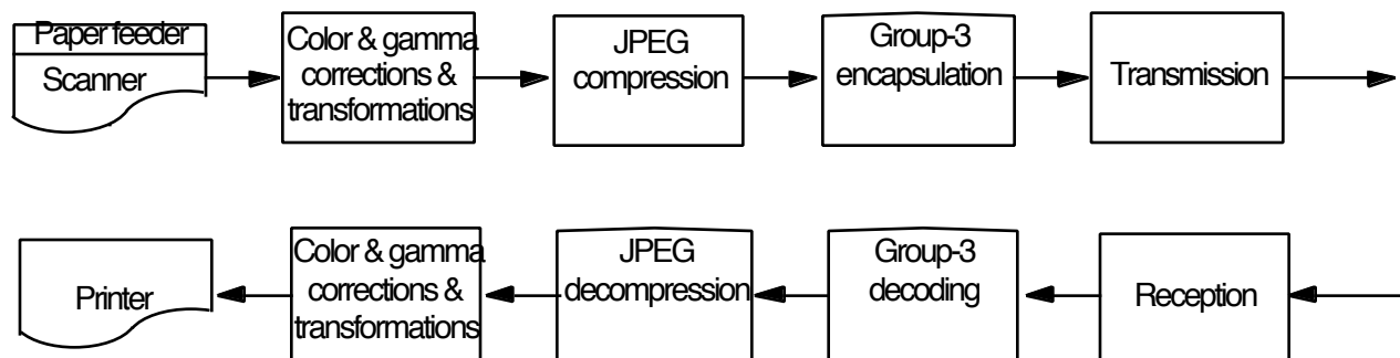
Figure 1. Color facsimile pipeline. The RGB bitmap is converted to the CIELAB color space and the chrominance channels are spatially subsampled. The image is then compressed using the JPEG method encapsulated for the conventional Group-3 facsimile protocol, and transmitted over an ordinary phone line. At the receiving end, the inverse operations are applied in reverse order.
