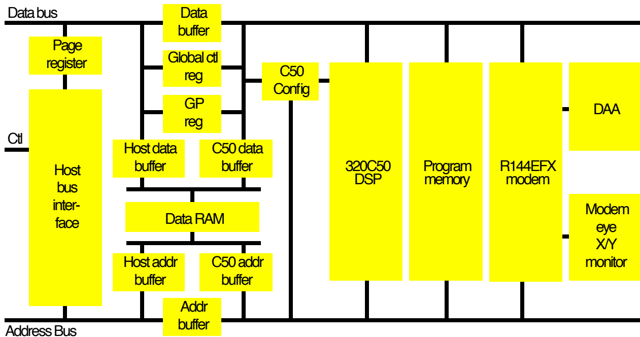
Figure 6. Block diagram of the DSP-based board for a color facsimile prototype.
