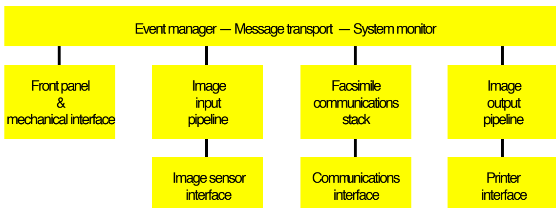
Figure 5. Block diagram of the software architecture.
