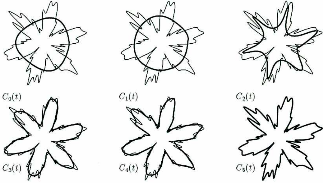
Figure 1: Six levels, C_i(t) , 0 \leq i \leq 5 , of the multiresolution decomposition of a B-spline star curve C_5(t) of order 3 defined using 100 control points. The original curve is shown in thin lines throughout while C_i(t) 's are shown in thick lines.
