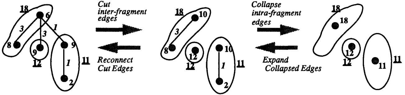
Figure 5: Connected Schedule as Cutting and Collapsing Edges
