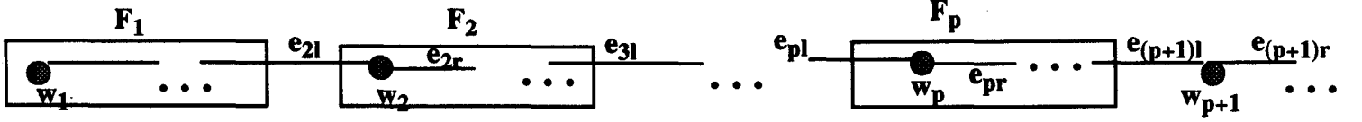
Figure 8: Fragments formed by BpSchedule before the last stage of BalancedCuts
