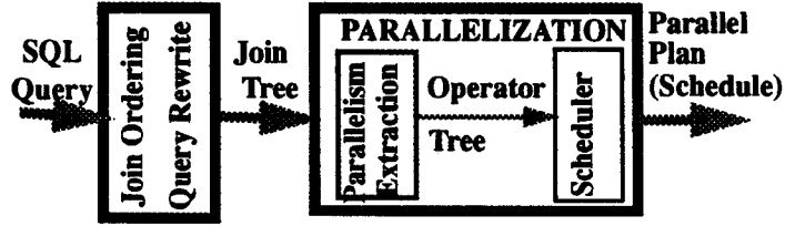
Figure 1: Two-phase Parallel Query Optimization
