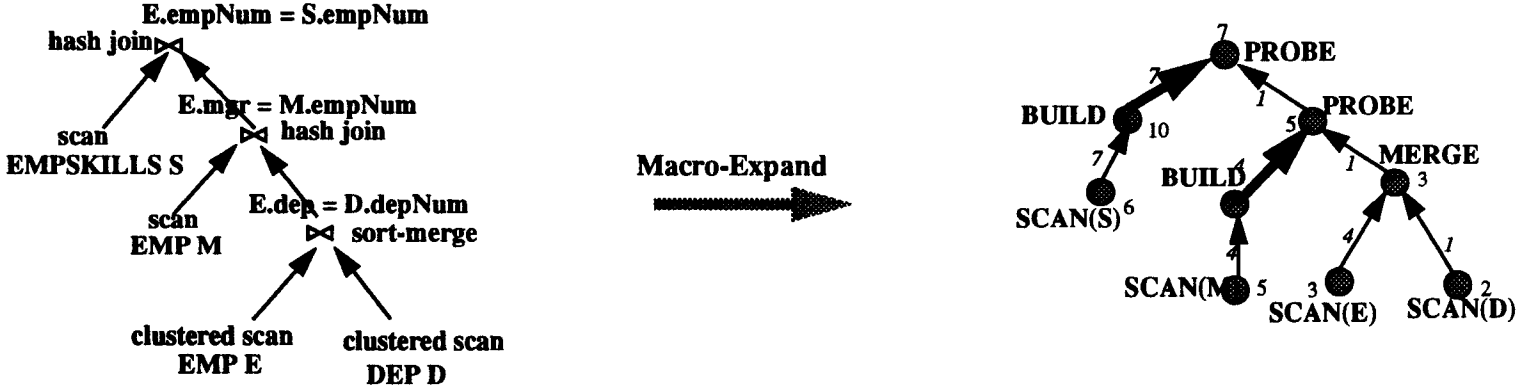
Figure 2: Macro-expansion of a Join Tree to a Weighted Operator Tree
