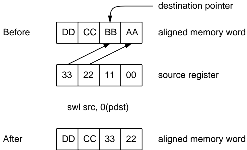
Figure 2: The Store Word Left instruction
