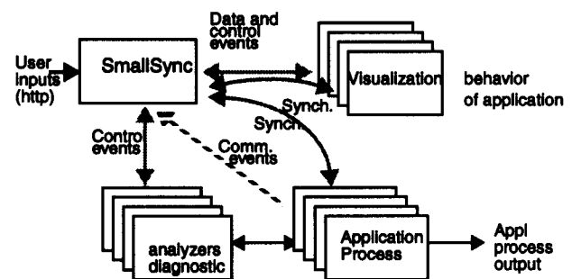
FIGURE 1. Architecture of SmallSync distributed process development and visualization environment.
