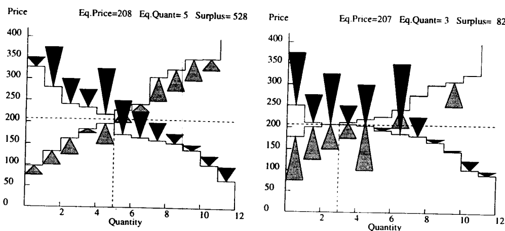
Figure 57: Bid-and-offer arrays in the experiment of Figure 52. Limit and shout prices are indicated using the triangles introduced in Figure 5. Left: at the start of Day 1. Right: at the start of Day 2.
