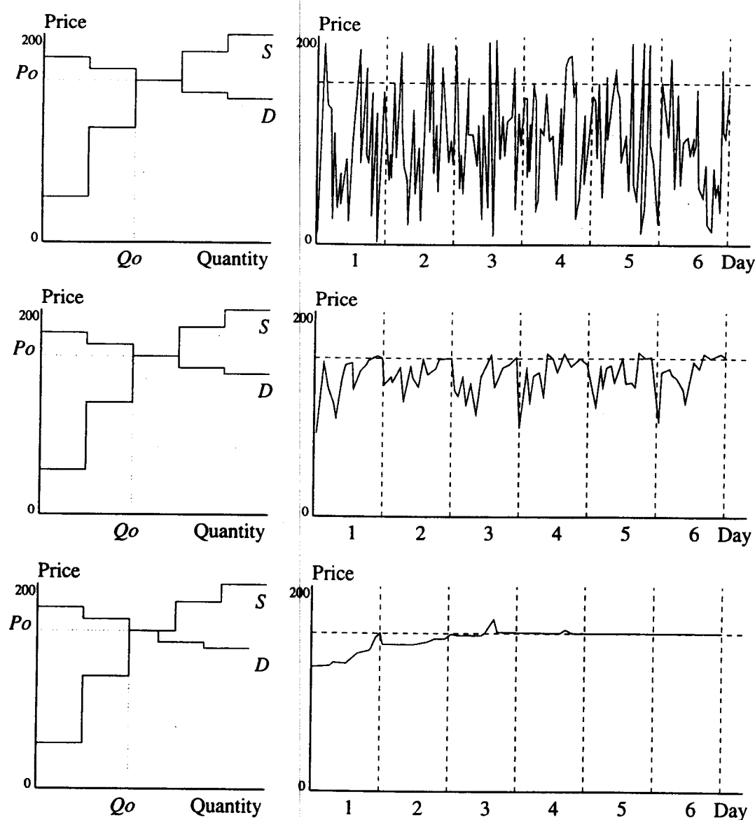
Figure 10: Typical results from one of Gode and Sunder's experiments (redrawn from Gode and Sunder (1993, Fig.4, p.127)). Top: results from ZI-U traders. Middle: results from ZI-C traders. Bottom: results from human traders. The figure to the left shows the supply and demand schedules for the experiment, the figure to the right shows the time series of transaction prices.
