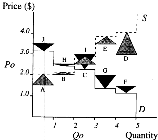
Figure 5: Bid-offer array for the ten-trader market illustrated in Figure 3, given random profit levels between zero and fifty percent. Each buyer's limit and shout prices are illustrated as dark inverted triangles, while each seller's limit and shout prices are illustrated by light upright triangles: the base of each triangle indicates the trader's limit price, while the apex indicates the trader's shout-price. The array of bid-prices gives an apparent demand curve D , and the array of offer-prices gives an apparent supply curve S . The apparent supply and demand curves differ significantly from the underlying supply and demand shown in Figure 3: see text for discussion.
