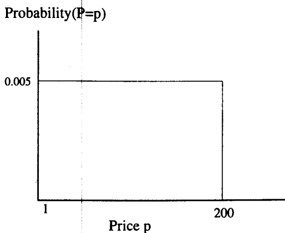
Figure 12: Probability density function (PDF) for prices 'shouted' by ZI-U traders: this PDF applies both to the sellers's offer-prices and the buyers' bid-prices.
