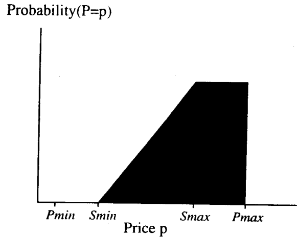
Figure 14: Qualitative probability density function (PDF) for ZI-C sellers: see text for discussion.
