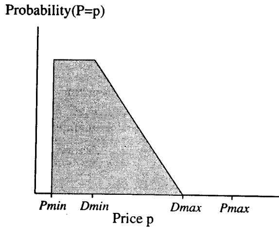
Figure 16: Qualitative probability density function (PDF) for ZI-C buyers: see text for discussion.
