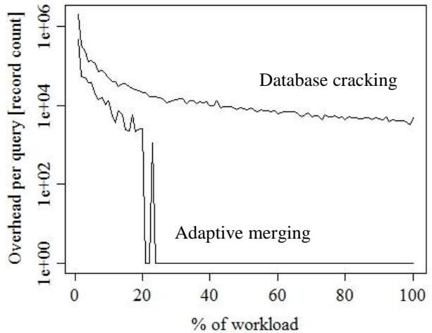
Figure 10. Small query ranges.
