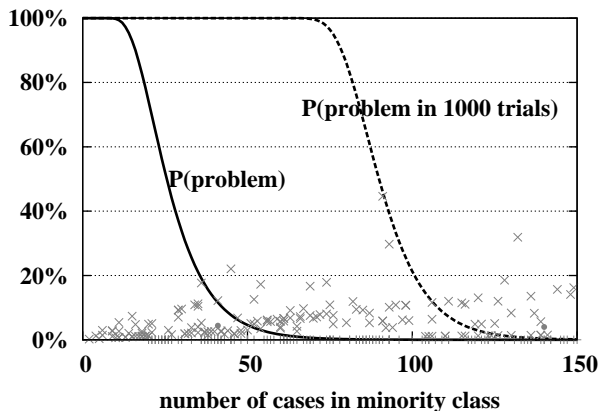
Figure 9: The probability of having at least one fold with no positives in 10-fold unstratified cross-validation, which results in undefined recall. The second curve shows this probability increasing given many independent trials: testing many different classes, many datasets to study, or random splits of the same dataset.
