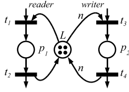
Figure 9. Reader-Writer Lock
