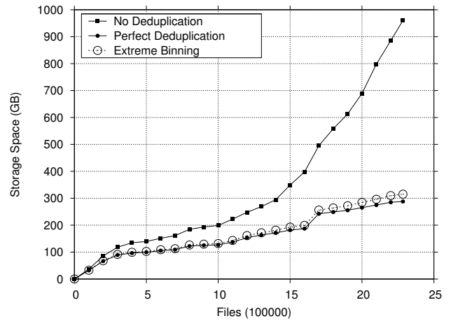
Fig. 6. Deduplication for LDup
