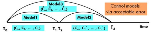
Figure 4. Model reconciliation.
