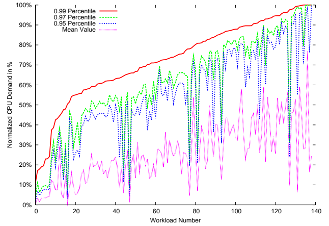
Fig. 2. Top Percentile of CPU Demand for Applications under Study.
