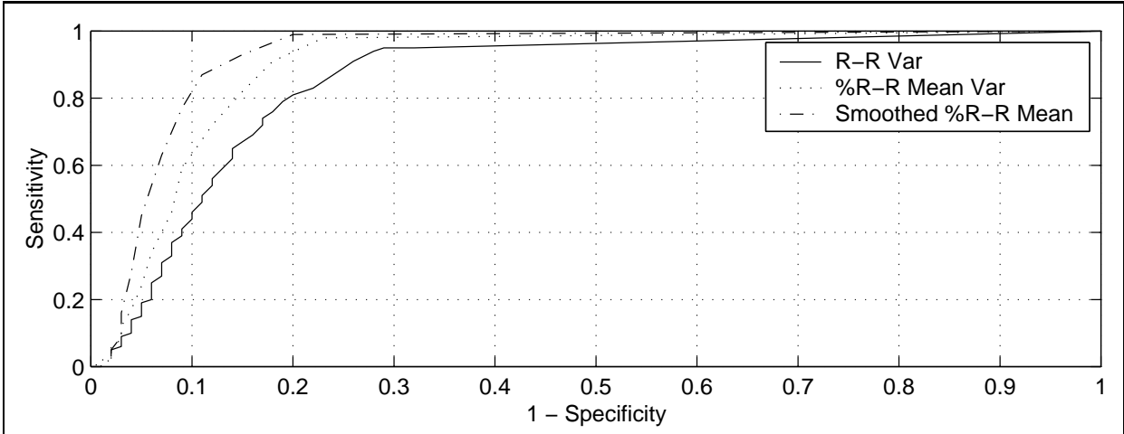
Figure 5: Results for 3 variants of our AF detection algorithm.
