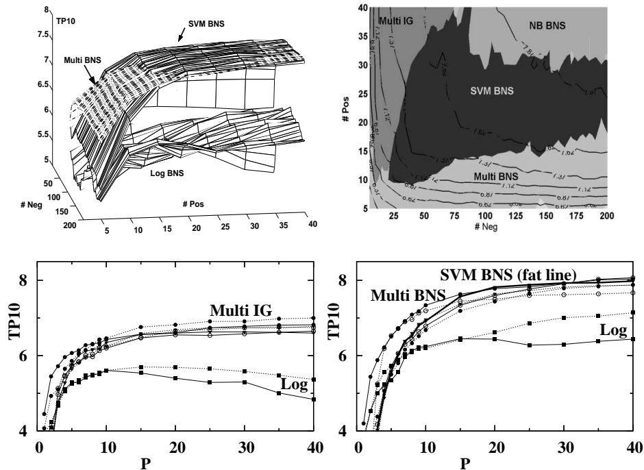
Fig. 2. TP10 performance. (a) Learning surfaces for three models (SVM-BNS, Multi-BNS and Log-BNS) as we vary the number of positives and negatives in the training set. (b) Topo-map of best models—3D surfaces of all models viewed from above. Isoclines show identical TP10 performance. (c) Cross-section at N=10 negatives, varying P positives. (d) Cross-section at N=200 negatives, varying P positives. (Legend in Fig.1.)
