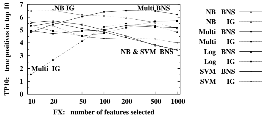
Fig. 1. Average TP10 performance for each learning model given P=5 positives and N=200 negatives, varying the number of features selected FX . (For more readable color graphs, see http://www.hpl.hp.com/techreports/2004/HPL-2004-19R1.html )
