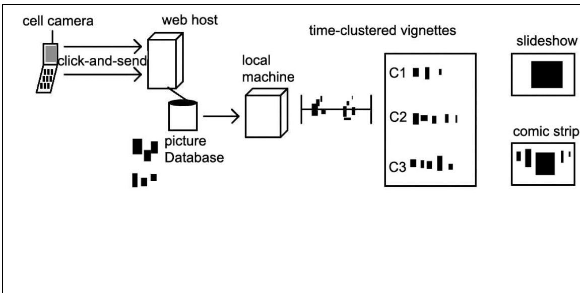
Figure 2: PLOG from picture capture to presentation
