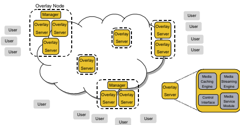
Figure 2: System architecture consisting of servers and managers.
