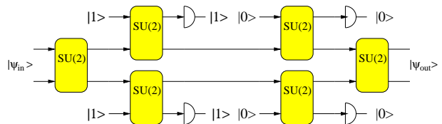
FIG. 6: Controlled- \hat{\sigma}_z gate with single-photon and vacuum detectors.
