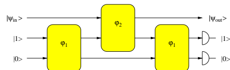
FIG. 1: Schematic setup of the KLM circuit for generating a nonlinear sign shift using 3 beam splitters, a single photon source and single photon resolving detectors.
