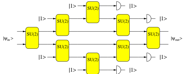
FIG. 5: Controlled-phase gate with single-photon detectors only.
