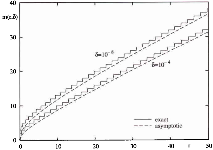
Figure 12: For the bounds \delta = 10^{-4} and \delta = 10^{-8} of the sum over Bessel functions (87) the result of the exact computation of m(r, \delta) (full curves) and the asymptotic result (96) are compared. The asymptotic results approaches the exact one slowly from below with a rate O(r^{-1/3}) .
