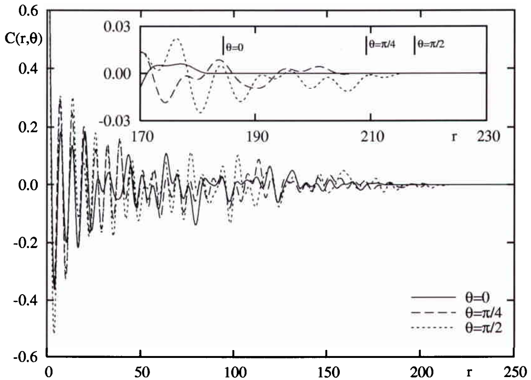
Figure 2: Autocorrelation function for the same state as fig. 1, but for a larger r -interval showing the non-universal behavior at larger r . The inset shows a magnification and the vertical bars indicate the places r = \sqrt{E_n} \text{diam}(\Omega, \theta) from where on C(r, \theta) = 0 , due to the compactness of the billiard.
