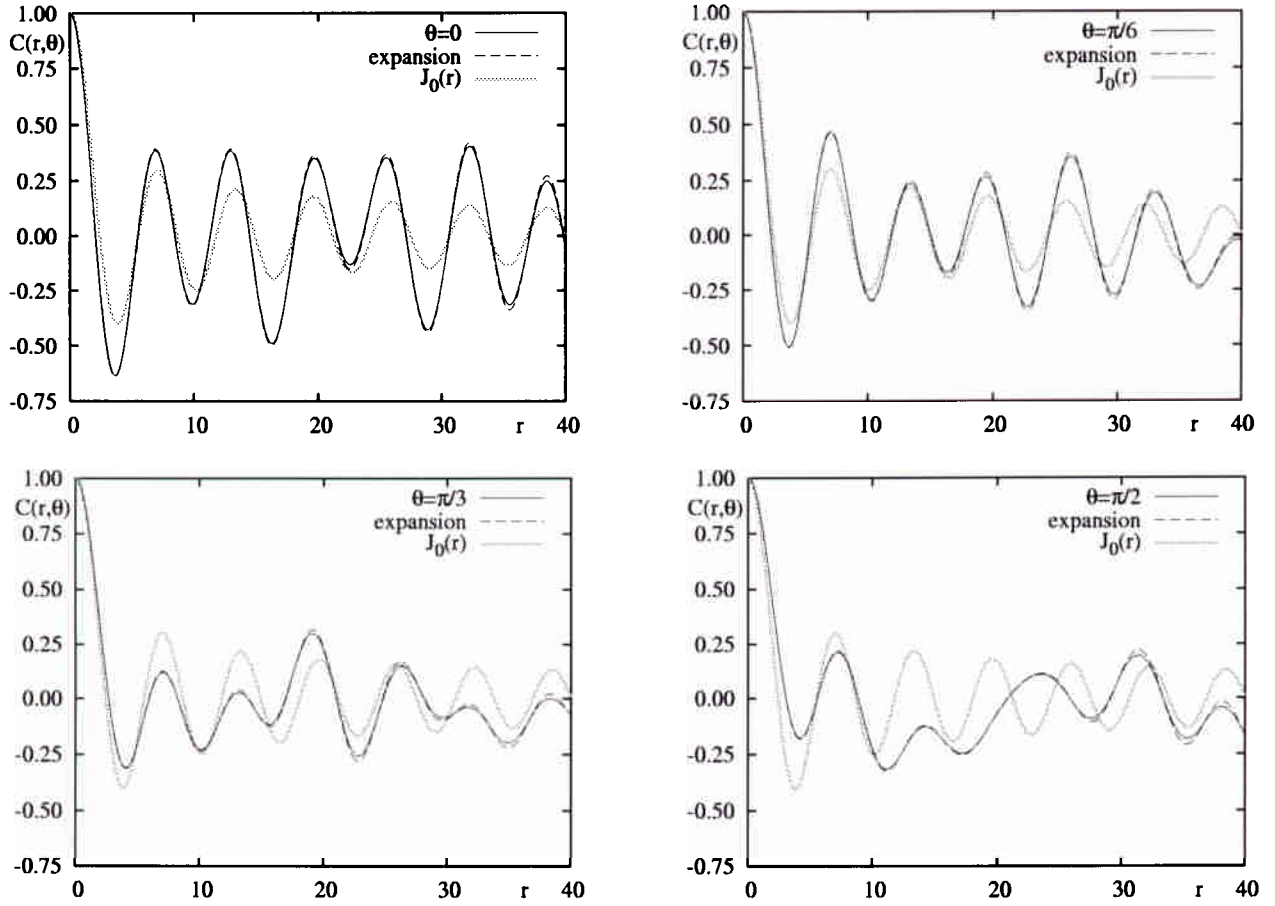
Figure 5: Comparison of the autocorrelation function C(r, \theta) for \psi_{1907} in the stadium billiard (full curve) with the expansion (33). In particular for small r the agreement is excellent, whereas for larger r small differences become visible.
