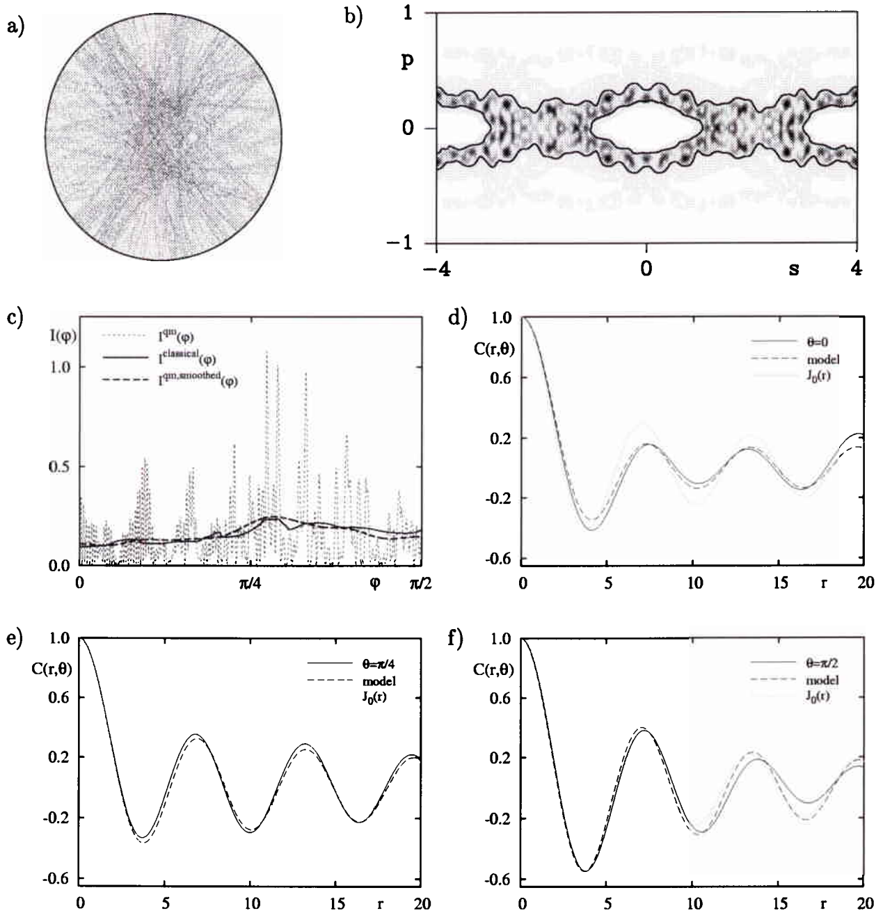
Figure 10: Autocorrelation function for a high lying irregular state ( E = 1002754.70\dots , approx. 130516^{\text{th}} eigenfunction of odd symmetry) in the limaçon billiard with \varepsilon = 0.3 . In b) the Husimi representation on the boundary is shown together with an approximate boundary (full line) of the region \mathcal{D} on which the state localizes. The resulting classical momentum distribution I^{\text{classical}}(\varphi) is shown in c) as full line and compared with the radially integrated momentum distribution I^{\text{qm}}(\varphi) of the state in a) and a smoothing of this, I^{\text{qm,smoothed}}(\varphi) , shown as dashed line. In d)–f) the autocorrelation function C(r, \theta) of the eigenfunction is compared for three different directions with result of the expansion (43) using I^{\text{classical}}(\varphi) .
