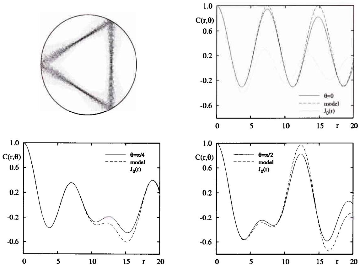
Figure 7: High lying eigenfunction ( E = 367984.82 \dots , approx. 47788 th eigenfunction of odd symmetry) in the limaçon billiard ( \varepsilon = 0.3 ), which localizes on the stable orbit of triangular shape. The autocorrelation function for three different directions is compared with the \delta -model, eq. (40), shown as dashed line using the directions of the stable orbit.
