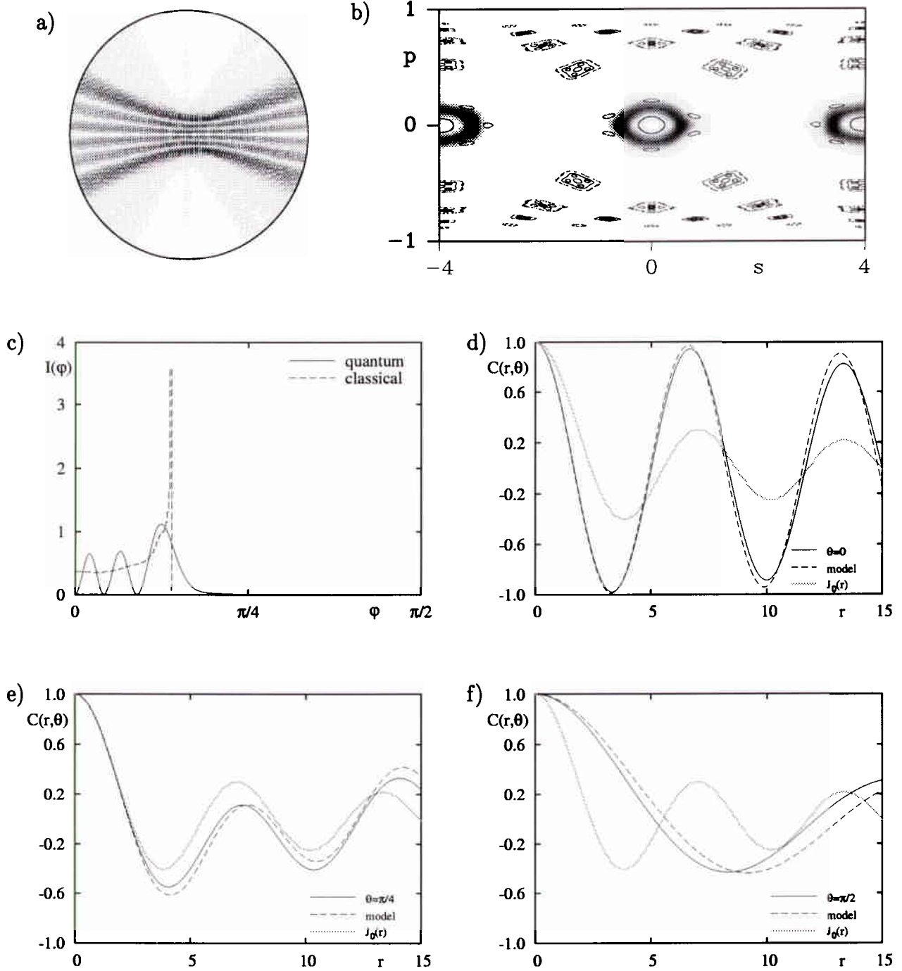
Figure 9: Grey scale plot of \psi_{3056} for the limaçon billiard with \varepsilon = 0.3 together with the corresponding Husimi plot, for which in addition some orbits are shown. In c) the radially integrated momentum distribution I_{3056}(\varphi) and the corresponding classical distribution I^{\text{classical}}(\varphi) for the torus are shown. In d)–f) the exact autocorrelation function is compared with the expansion of the autocorrelation function, eq. (33), using I^{\text{classical}}(\varphi) for different angles \theta .
