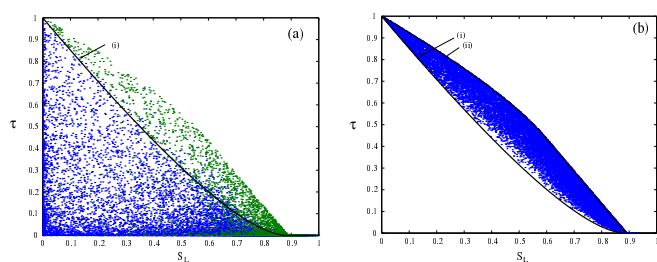
FIG. 1: Plot of the tangle, \tau , and linear entropy, \mathcal{S}_L , of numerically generated two-qubit random matrices. Two sets of data are plotted: a) 30,000 randomly generated matrices, which show the extent of physical states in the entanglement-purity plane; b) 30,000 randomly generated matrices weighted to explore the boundary region. Also shown are analytical curves for: i) the Werner state, a mixture of the maximally-entangled state and the maximally-mixed state; and ii) the maximally-entangled mixed states, states with the maximal amount of entanglement for a given degree of linear entropy (or vice versa). See text for further details.
