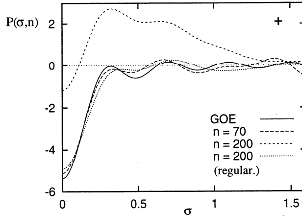
FIG. 5. The periodic orbit correlation function shown for various n - values in the ‘+’ subspace with enhanced resolution compared to Fig. 4; the regularisation procedure (35) eliminates the exponentially growing terms and universal correlations are uncovered now also for n = 200 .
