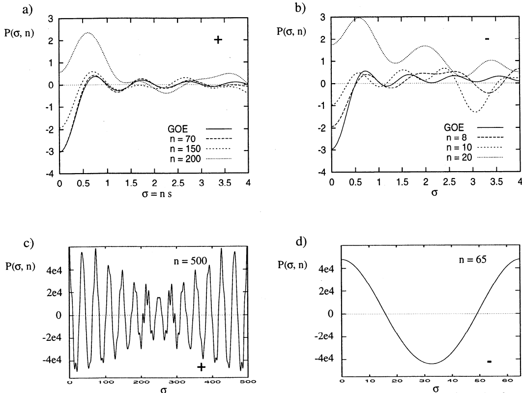
FIG. 4. The periodic orbit correlation functions are shown for various n - values in the '+' subspace (Fig. a, c) and '-' subspace (Fig. b, d); 'universal' periodic orbit correlation which coincide with the GOE - prediction can be observed up to n \approx 70 in the '+' subspace, but only up to n \approx 8 in the '-' subspace. Non-universal periodic orbit correlations develop for large n (with exponentially increasing amplitude), see Fig. c and d. The cut-off is N_{\max} = n here, see Eq. (32).
