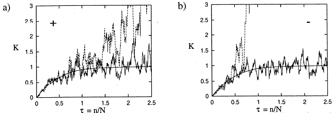
FIG. 3. The form factor K(\tau) , i.e. the square modulus of the quantum traces \text{Tr}\tilde{U}^n (full line) and the semiclassical traces \text{Tr}\tilde{U}^n (dashed line) for positive (a) and negative (b) parity is displayed as function of \tau = n/N for N/2 = 259 together with the RMT - result for the Gaussian Orthogonal Ensemble (smooth curve). The semiclassical break-times, Eq. (31), are \tau_b^+ \approx 1.002 , \tau_b^- \approx .301 , respectively.
