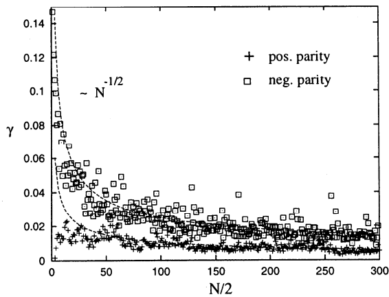
FIG. 2. The semiclassical eigenvalue with the largest modulus plotted here as \gamma^{\pm}(N) = \log |\Lambda_0^{\pm}(N)| versus N/2 for both subspaces; the deviation from the unit circle decreases in both cases like 1/\sqrt{N} (dashed lines), but one finds typically \gamma^+(N) < \gamma^-(N) .
