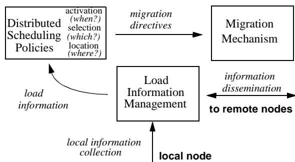
Figure 4: Load Information Management Module collects load information on local node and disseminates it among the nodes. Distributed Scheduling instructs the migration mechanism when, where, and which process to migrate.
