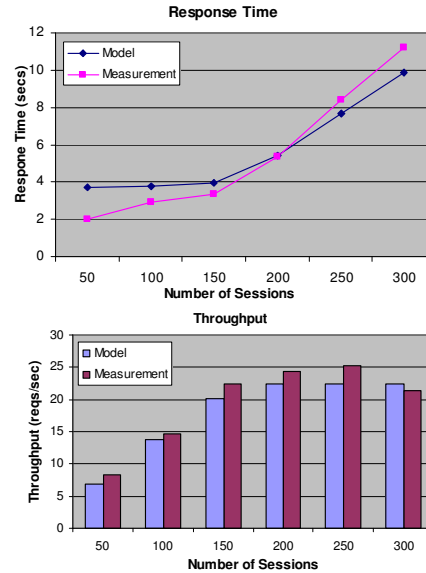
Figure 8. RUBiS performance
