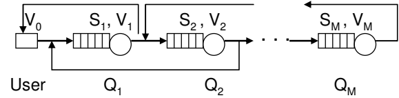
Figure 3. Basic queuing network model
