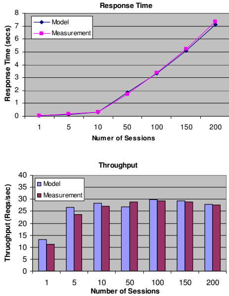
Figure 7. TPC-W performance
