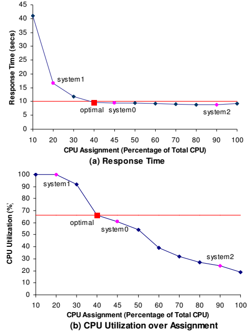
Figure 10. Performance of RUBiS in a virtualized data center
