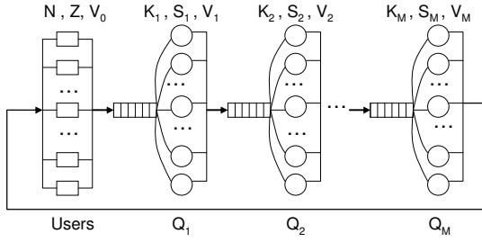
Figure 4. Closed multi-station queueing network
