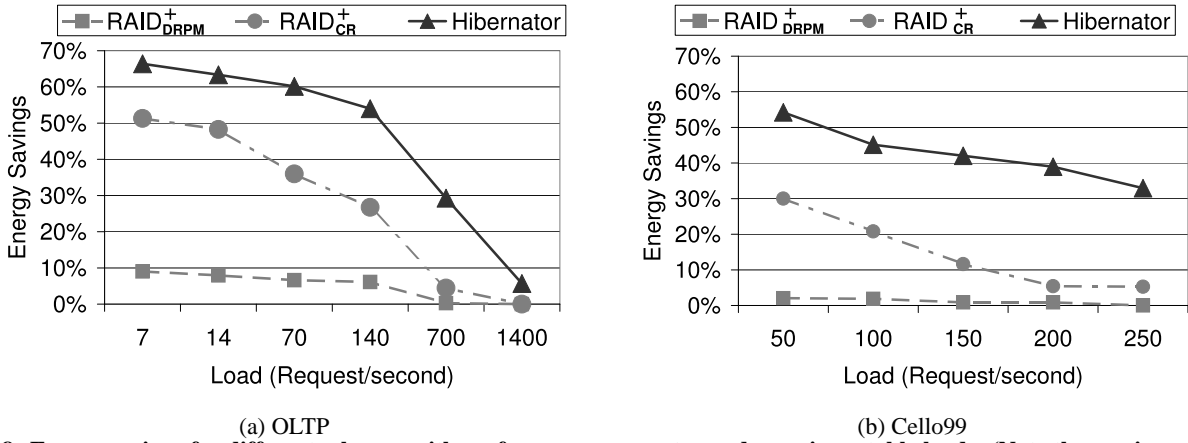
Figure 8: Energy savings for different schemes with performance guarantee under various stable loads. (Note the x-axis scale in (a) is not linear.)
