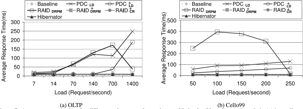
Figure 7: Average response time for different schemes under various stable loads. (Note the x-axis scale in (a) is not linear.)
