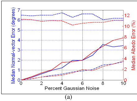
Figure 4: (a): Solid lines: Noise sensitivity for robust PTM estimate of surface normal and albedo. Dot-dashed lines: robust PST – using weights w^0 generated by robust PTM. Dashed lines: standard PST. (b): Synthetic sphere with 10% noise. (c): Noise contribution (positive values shown).
