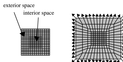
Figure 7. Volumetric Warping. Pre-warped (left) and warped (right) voxel spaces are shown in two dimensions. The voxel space is divided into two regions; an interior space shown with dark gray voxels, and an exterior space shown with light gray voxels. Before the warping is applied, both regions consist of voxels of uniform size. The warping does not affect the voxels in the interior space, while the voxels in the exterior space increase in size further from the interior space. The outer shell of voxels in the warped voxel space gets warped to infinity. These voxels are represented with arrows in the figure.
