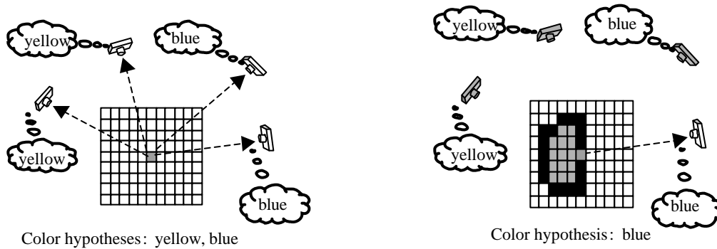
Figure 6. Multi-hypothesis voxel coloring. Hypothesis assignment for a voxel is shown on the left, where the striped voxel is projected into each image, and hypotheses are stored for the voxel. On the right, hypotheses that are inconsistent with the active camera's observation are removed. (The active camera is given a white color). Hypothesis removal considers the visibility of the scene. Thus, for the configuration of the voxel space on the right, the cameras that observe yellow for the voxel will not be considered.
