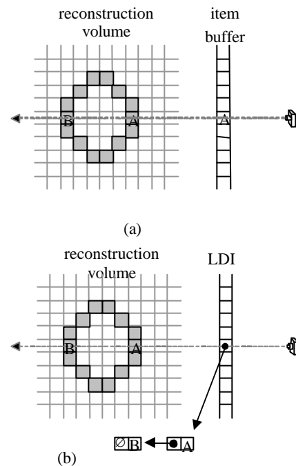
Figure 4. The two variants of GVC use different data structures, called item buffers and layered depth images (LDIs), to compute the visibility of voxels. In (a), an item buffer records, for every pixel in an image, the surface voxel that is visible from the pixel. In (b), an LDI records, for every pixel in an image, a depth-sorted list of all surface voxels that project to the pixel.
