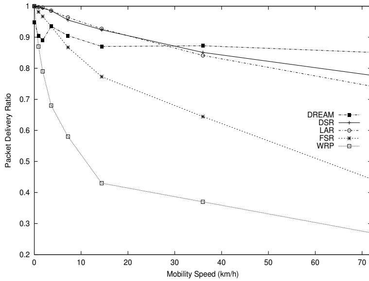
Figure 1: Average Packet Delivery Ratio as a Function of Mobility Speed.
