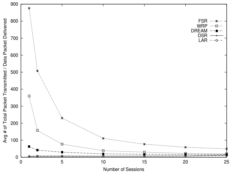
Figure 7: Average Number of Total Packets Transmitted per Data Packet Delivered as a Function of Number of Sessions.
