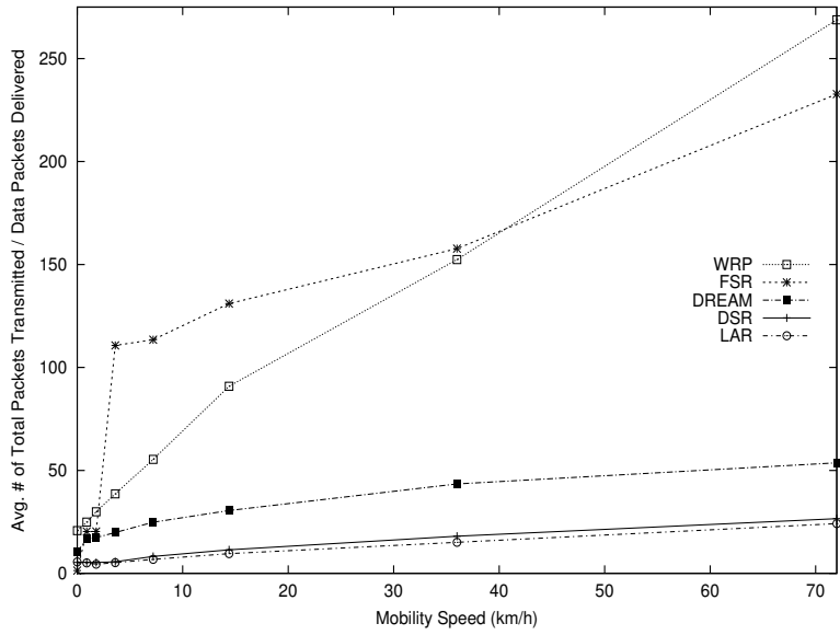
Figure 5: Average Number of Total Packets Transmitted per Data Packet Delivered as a Function of Mobility Speed.
