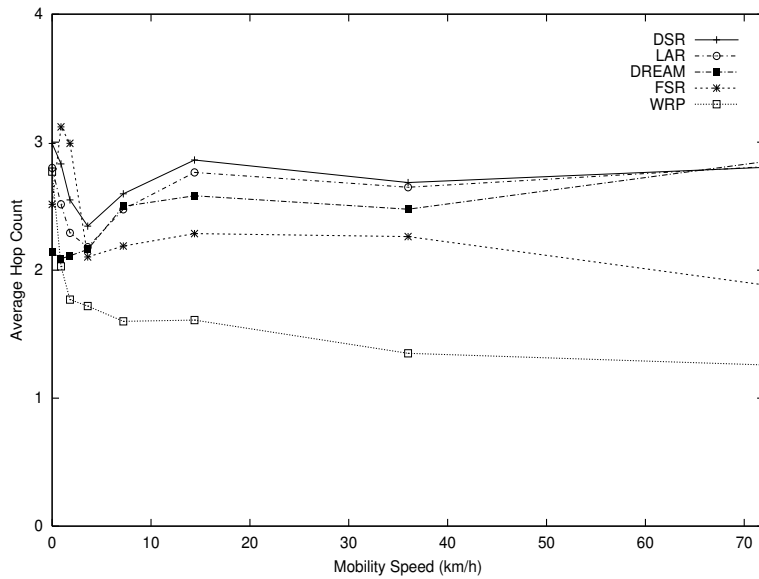
Figure 2: Average Hop Count as a Function of Mobility Speed.
