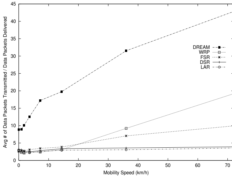
Figure 3: Average Number of Data Packets Transmitted per Data Packet Delivered as a Function of Mobility Speed.
