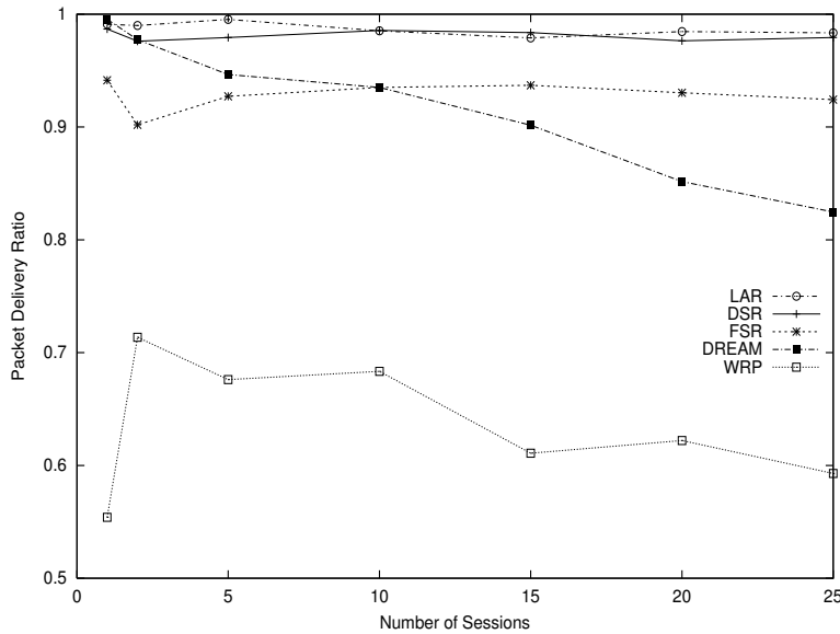
Figure 6: Average Packet Delivery Ratio as a Function of Number of Sessions.
