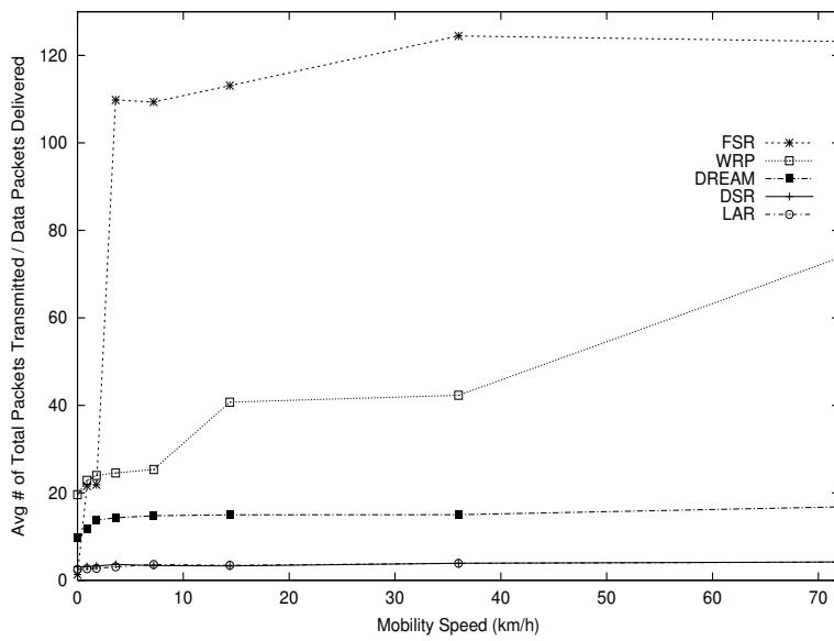
Figure 9: Average Number of Total Packets Transmitted per Data Packet Delivered as a Function of Group Mobility Speed.
