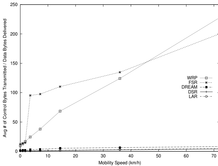
Figure 4: Average Number of Control Bytes Transmitted per Data Byte Delivered as a Function of Mobility Speed.
