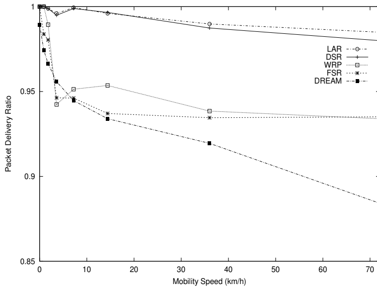
Figure 8: Average Packet Delivery Ratio as a Function of Group Mobility Speed.
