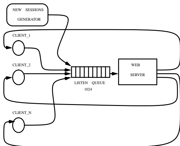
Figure 1: Basic Structure of Simulation Model.
