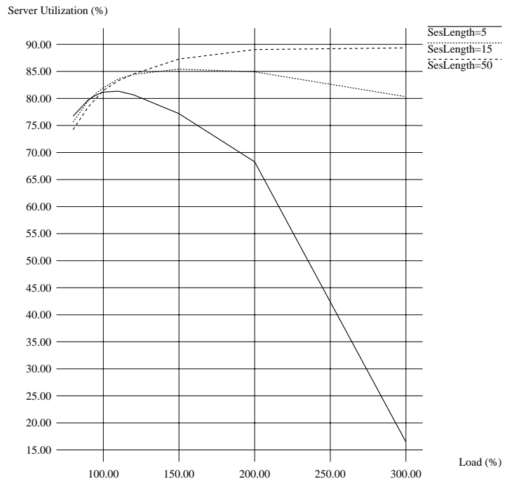
Figure 9: Useful Utilization for a Server with Admission Control.
