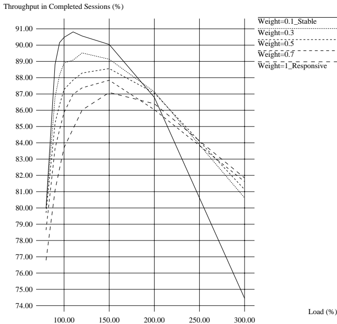
Figure 12: Throughput in Completed Sessions for Family of AC-Functions: from AC-Stable to AC-Responsive, Workload with Average Session Length of 15.
