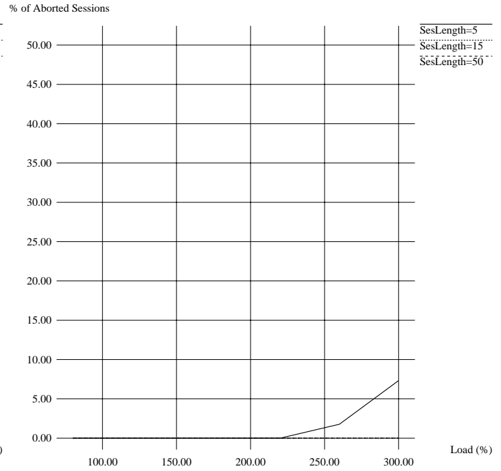
Figure 11: Percentage of Aborted Sessions from Admitted for Processing for Server with Admission Control, AC-Interval = 0.5sec, Workload with Average Session Length of 5.
