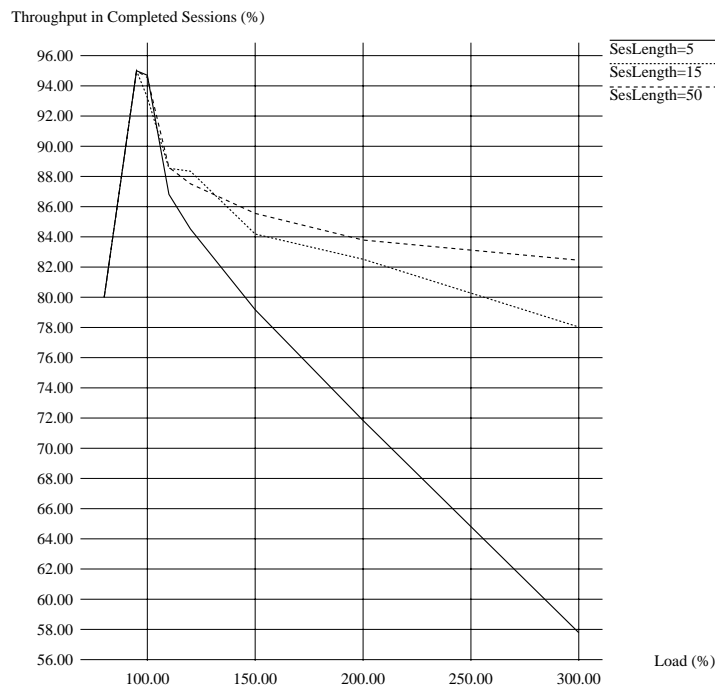
Figure 2: Throughput in Completed Sessions for Overloaded Server.
