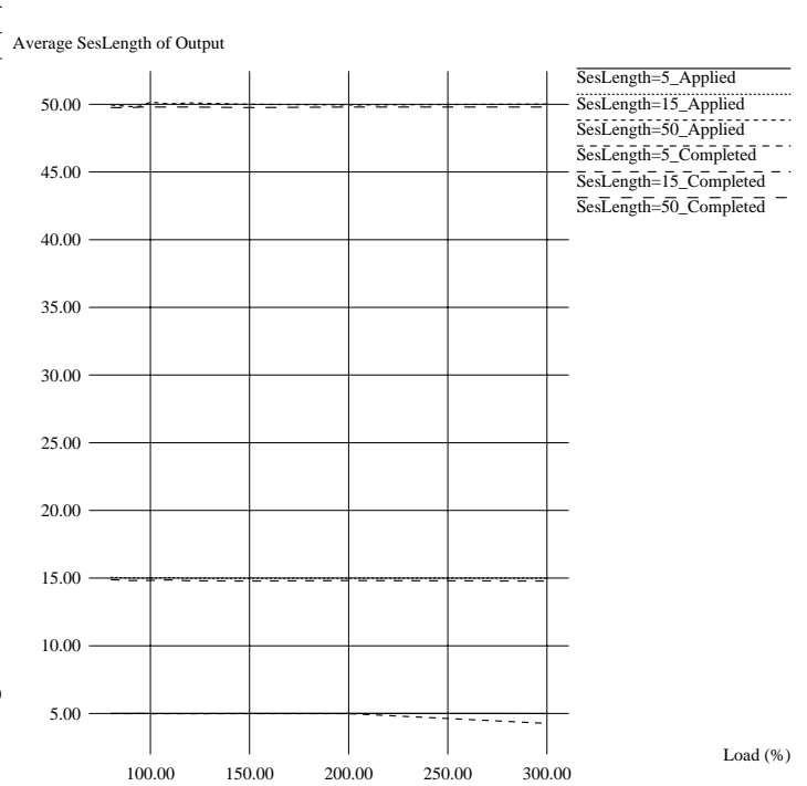
Figure 8: Average Length of Completed Sessions by Overloaded Server with Admission Control.
