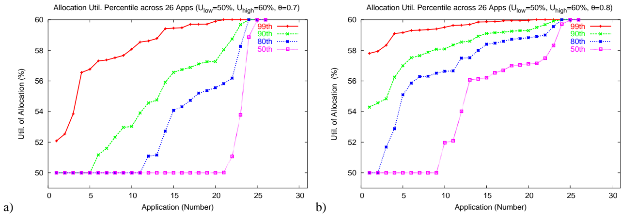
Figure 3: Distribution of Application Utilization of Allocation.
