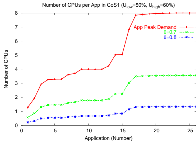
Figure 2: Application Workload Usage of CoS 1.
