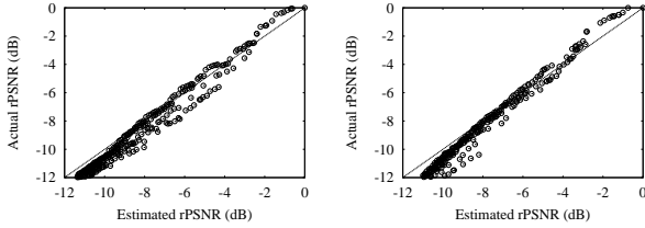
Figure 3: The robustness of the rPSNR metric in video quality estimation: Foreman , H.264 coding (left), and Mother & Daughter , MPEG-2 coding (right).
