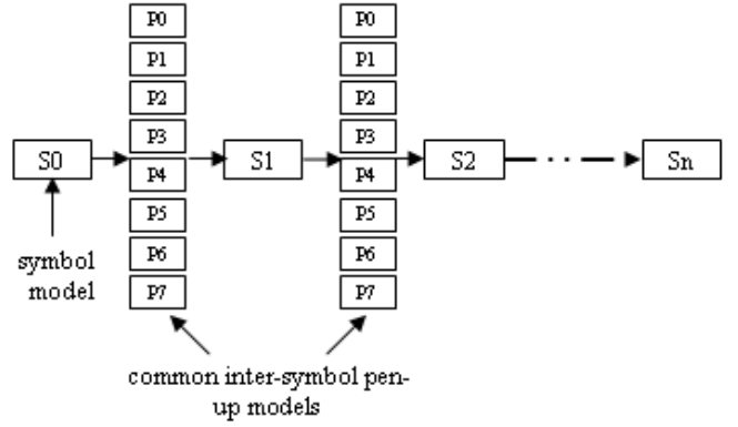
Figure 4. Word network with explicit inter-symbol pen-up models
