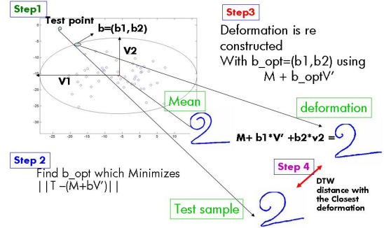
Figure 1. Illustration of the recognition process for the Active-DTW classifier
