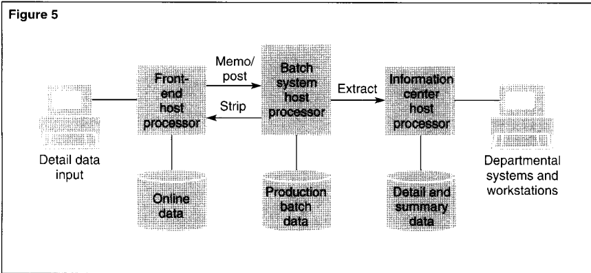
Figure 5. Typical information processing architecture. The information center data consists of detail plus weekly, monthly, or other summary data.
