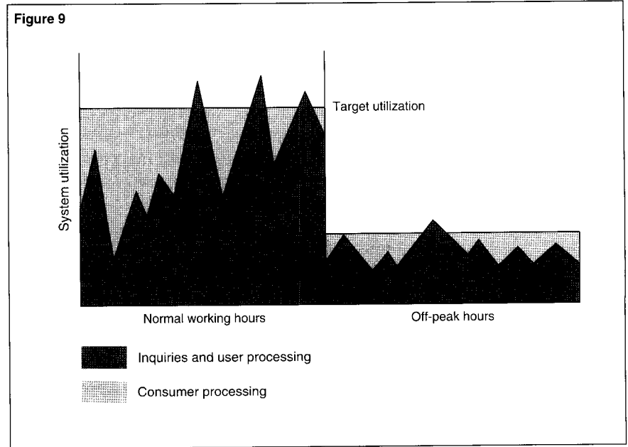
Figure 9. RESPOND consumers use spare CPU cycles without impacting user response time.
