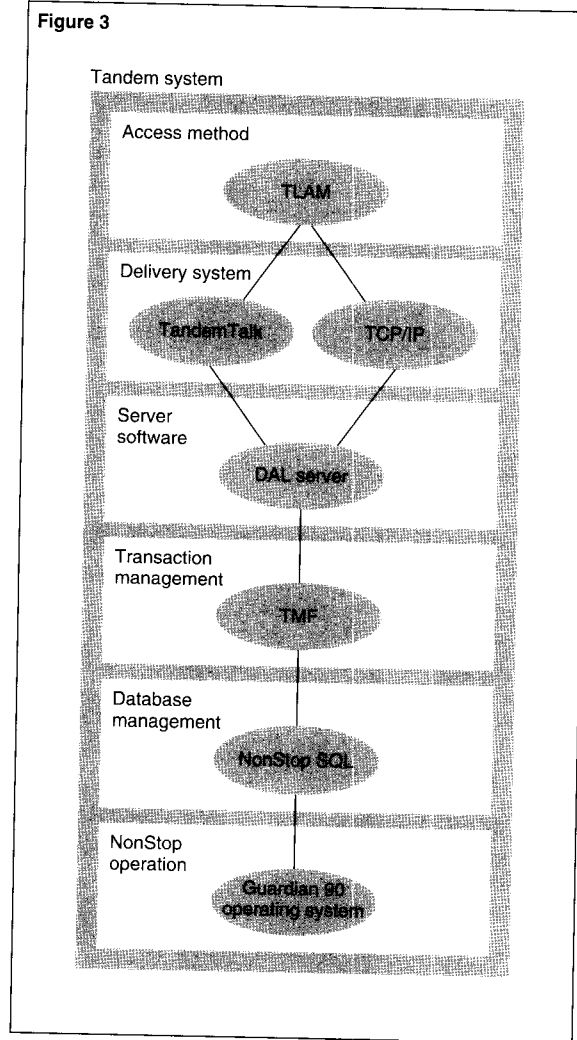
Figure 3. The DAL Server in the Tandem environment.
