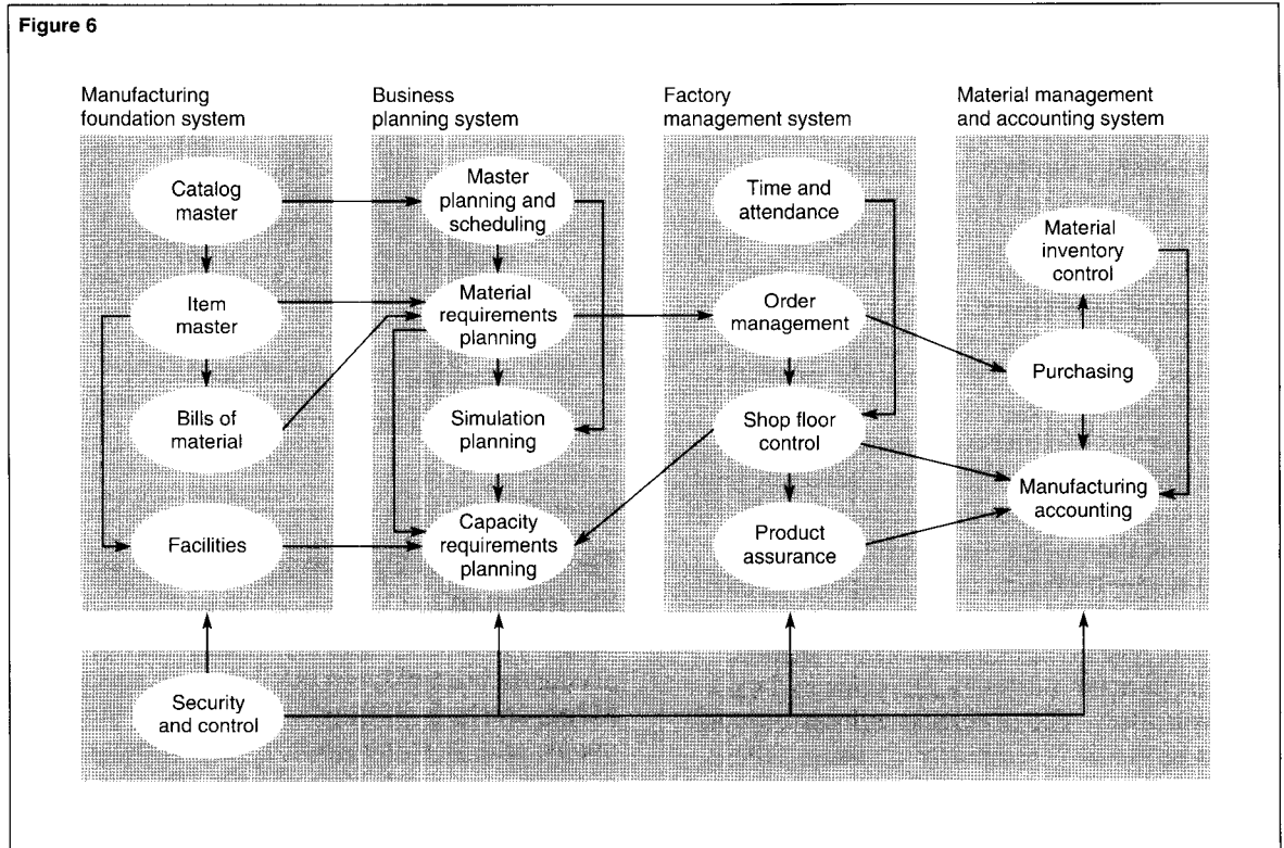
Figure 6. RESPOND is a modular application.
