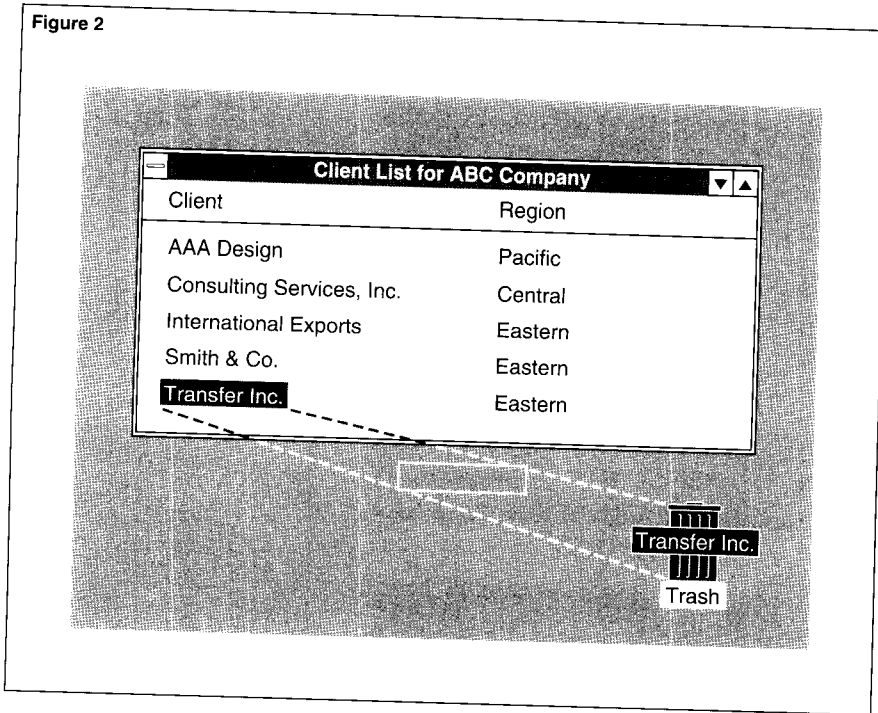
Figure 2. Drag-and-drop operations.
