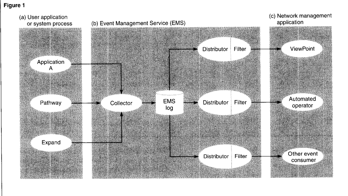
Figure 1. Event management in the DSM environment. (a) A user application or system process performs event generation. (b) EMS performs event collection and distribution. (c) A network management application performs event consumption.
