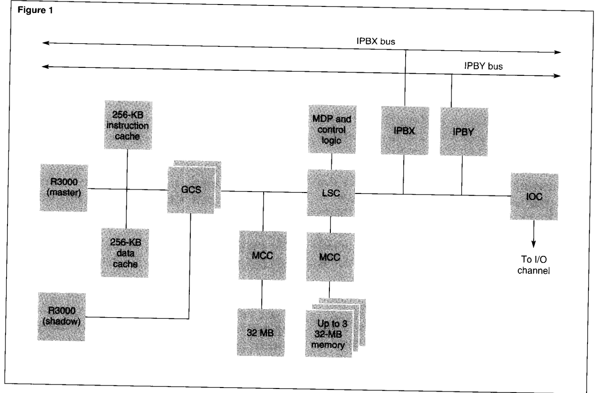
Figure 1. Block diagram of TNS/R CPU board.
