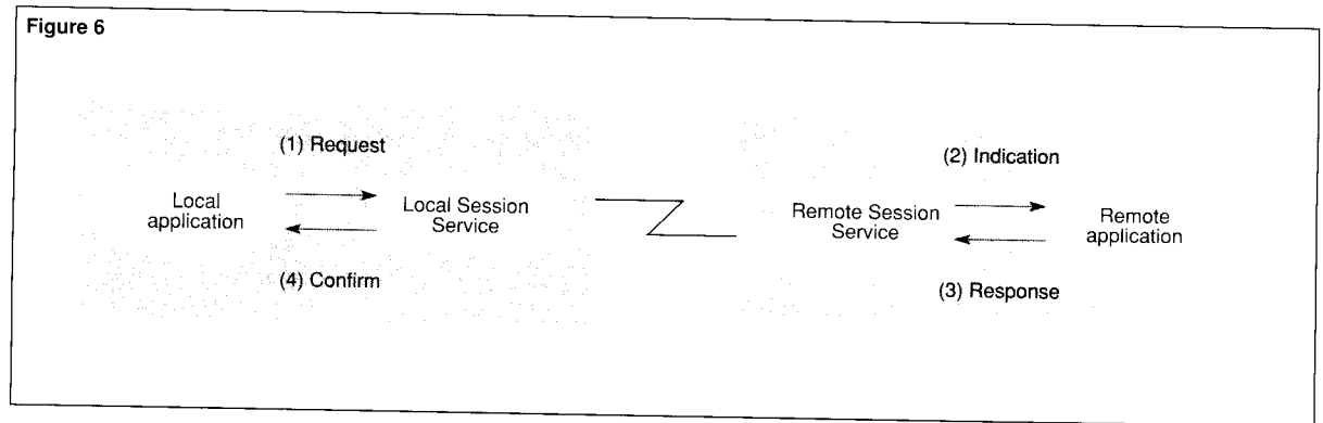
Figure 6. The four types of Session Layer primitives.
