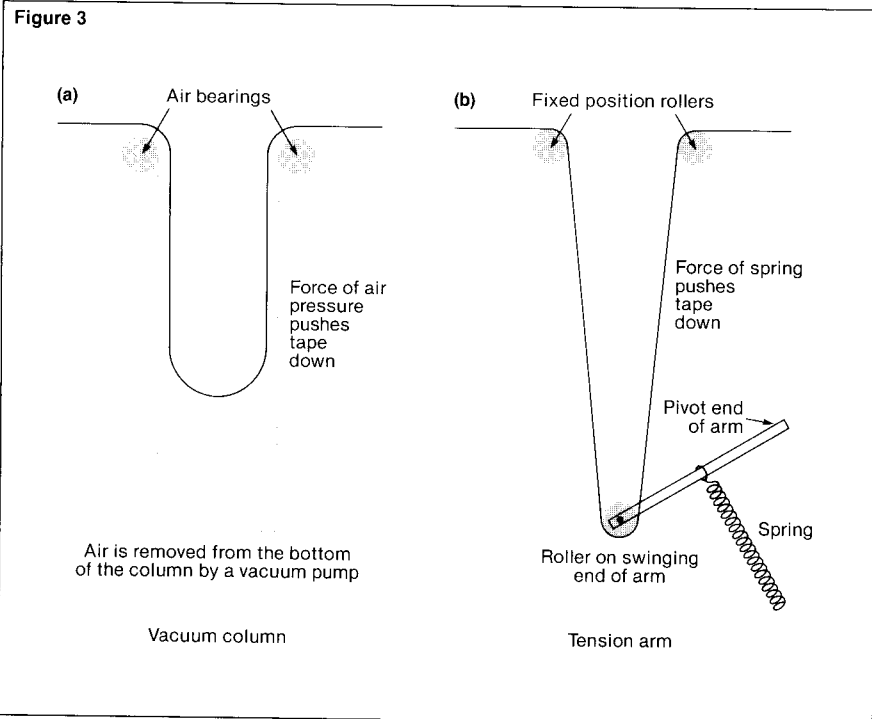
Figure 3. (a) A vacuum column uses air pressure to put tension on the tape. (b) A tension arm uses a spring-loaded arm to put tension on the tape.
