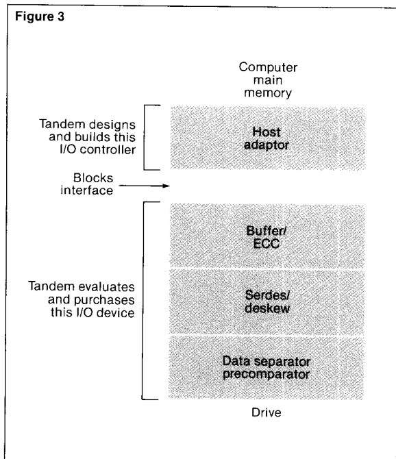
Figure 3. Example of division of I/O subsystem between a Tandem 3209 cartridge tape controller and device.
