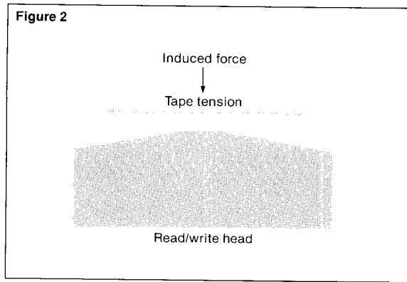
Figure 2. The tape tension and the wrap angle around the head induce a force which holds the tape against the head.
