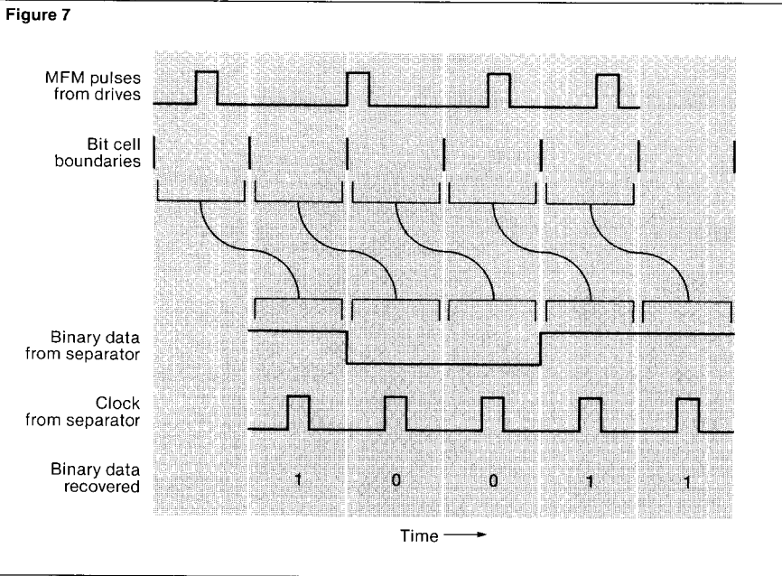
Figure 6. Example of MFM data encoding.
