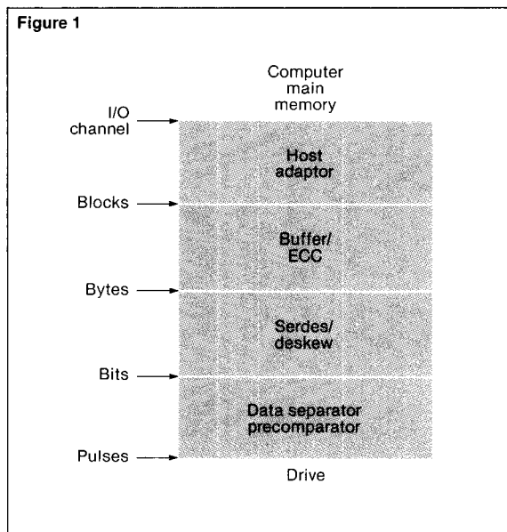
Figure 1. Model of I/O subsystem with computer and drive. The names of the interfaces of the subsystem correspond to the form in which information is transferred.
