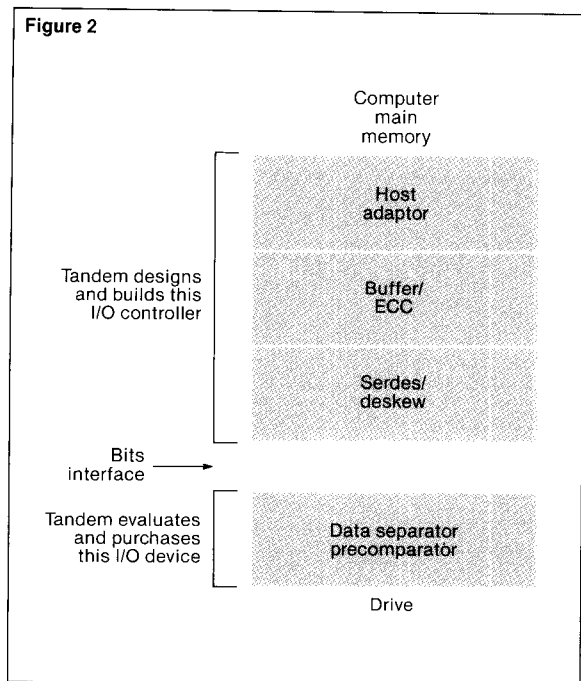
Figure 2. Example of division of I/O subsystem between a Tandem 3108 disk controller and device.
