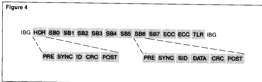
Figure 4. Physical data block.
