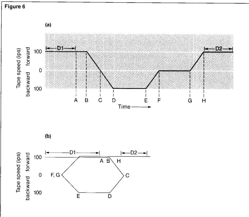
Figure 6. Repositioning. (a) Tape speed changing with time. (b) Tape position changing with time.
