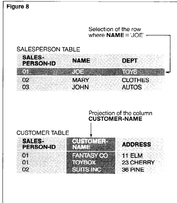
Figure 8. Projection selects columns; selection selects rows.
