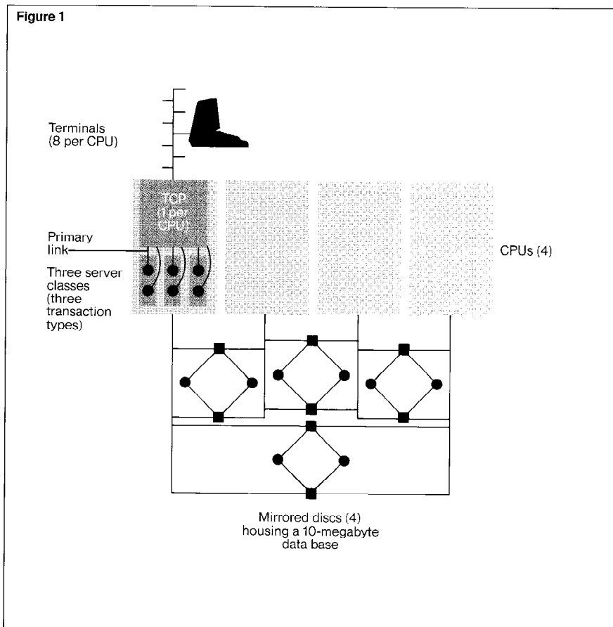
Figure 1. Configuration of hardware and software used in benchmark tests.
