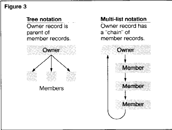
Figure 3. Link-sets can be represented graphically by the tree notation or the multi-list notation.
