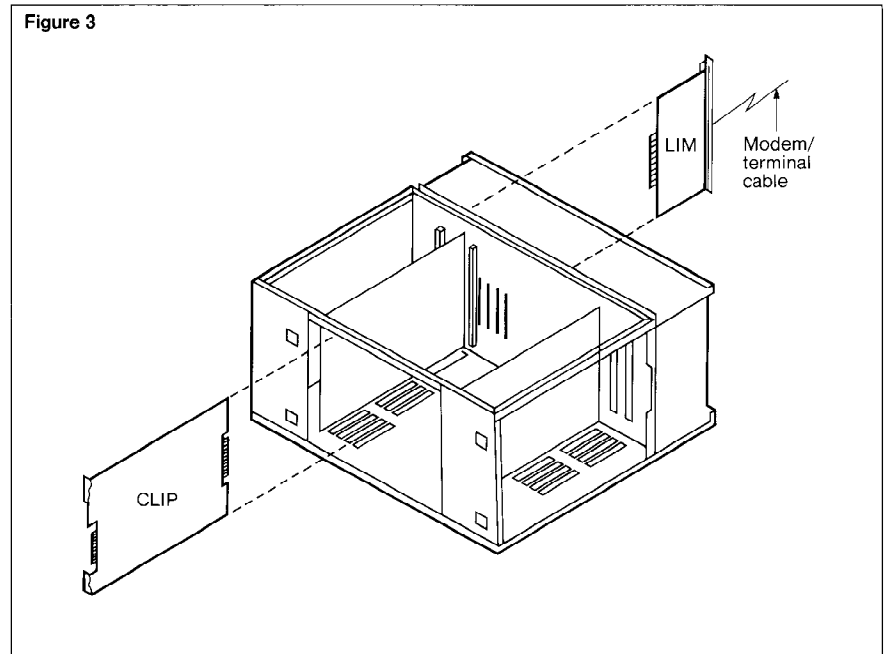
Figure 3. 6100 CSS card cage assembly.
