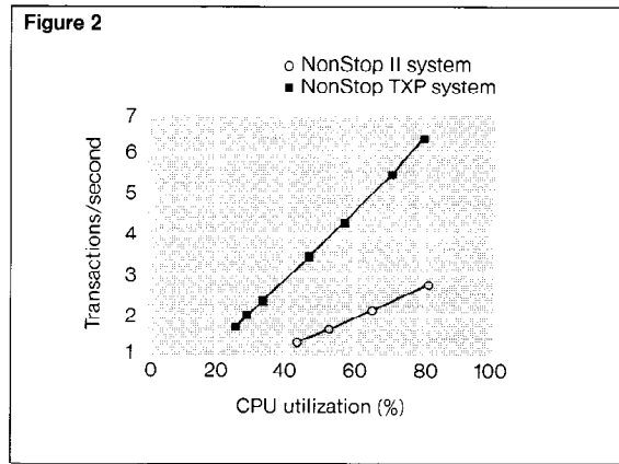
Figure 2. Measured levels of CPU utilization at various transaction rates.
