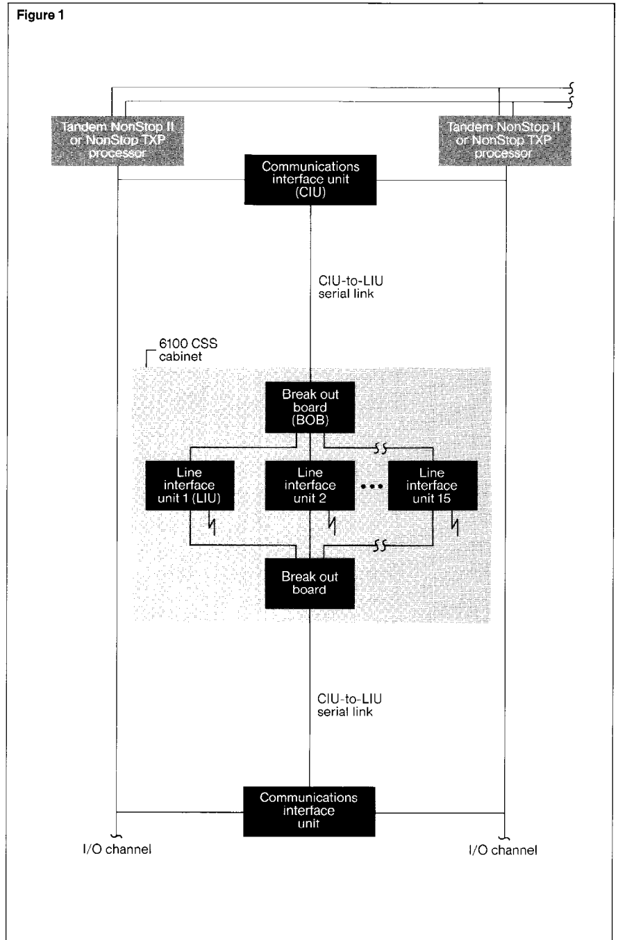
Figure 1. 6100 Communications Subsystem hardware components.
