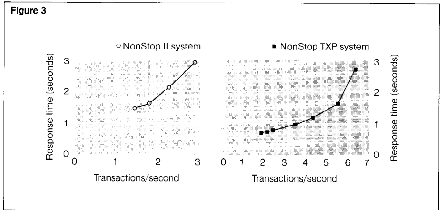
Figure 3. Measured response times at various transaction rates. Left: NonStop II. Right: NonStop TXP.
