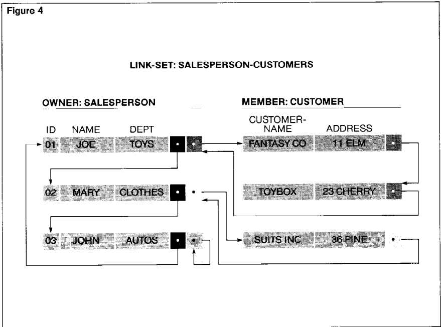
Figure 4. A link-set in the network data model, representing the relationship of a salesperson to many customers.
