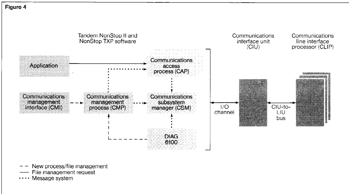
Figure 4. Major 6100 CSS software components.
