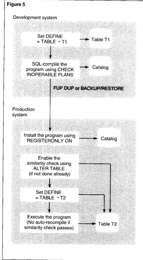
Figure 5. Scenario 1: Moving a program from development to production without SQL-compilation.
