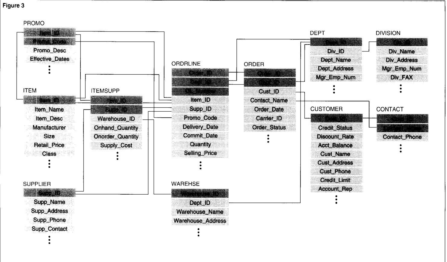
Figure 3. Tables and columns in a simplified OLTP order-entry database.
