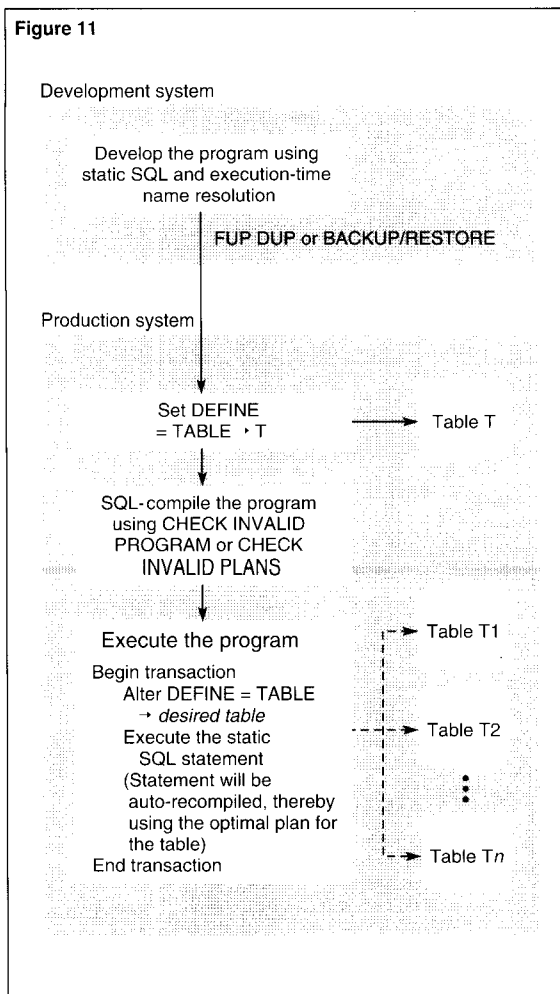
Figure 11. Scenario 7: Switching between databases and always using the optimal plan.
