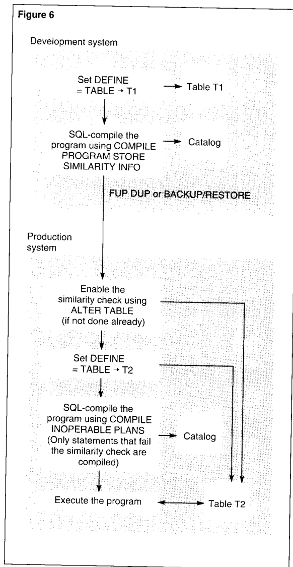
Figure 6. Scenario 2: Moving a program from development to production with minimal SQL-compilation.
