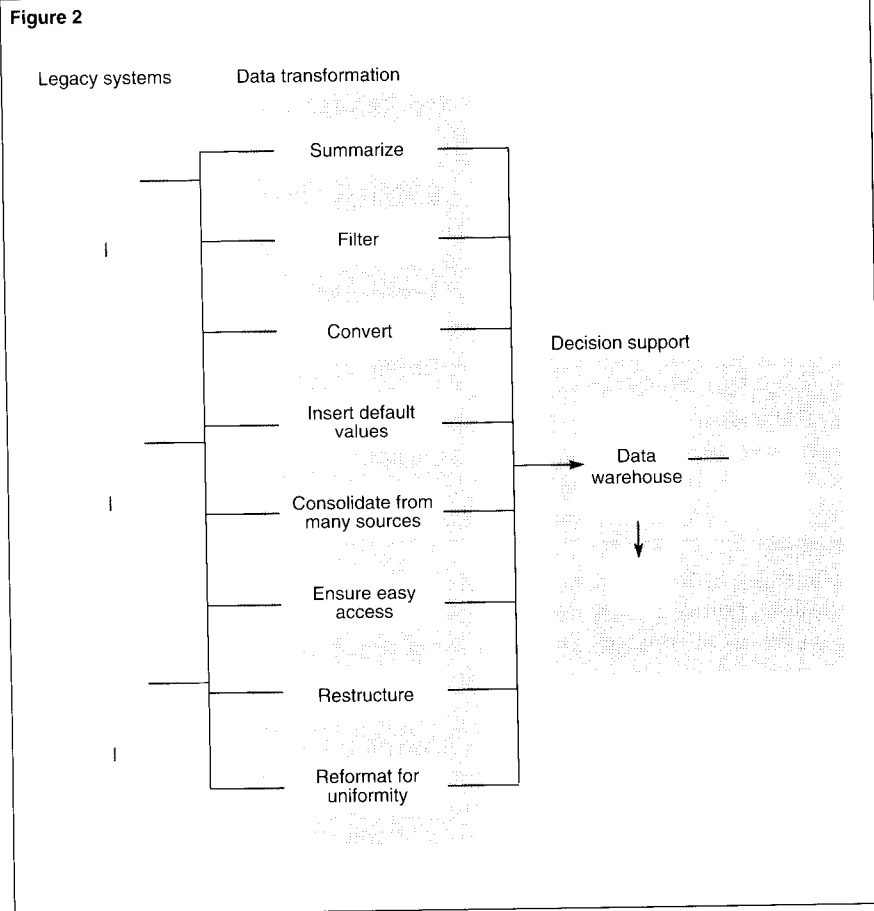
Figure 2. Components of data transformation that must take place before data is loaded into the data warehouse.
