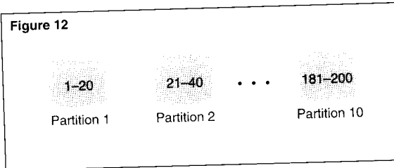
Figure 12. Partition table with 10 partitions for use with a fact table of 200 partitions.
