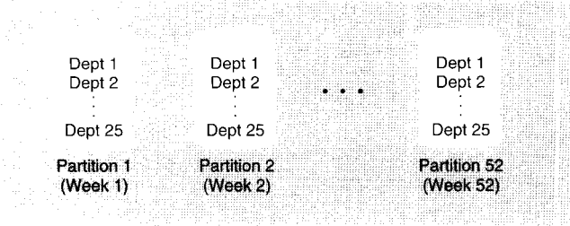
(a) Partitioning on Date, with Department as the second key column
