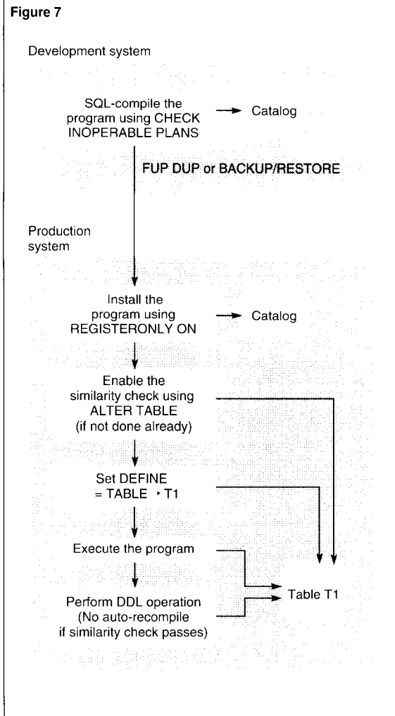
Figure 7. Scenario 3: Avoiding unnecessary auto-recompilations after a DDL operation.
