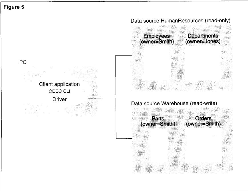
Figure 5. Client connections to two data sources.
