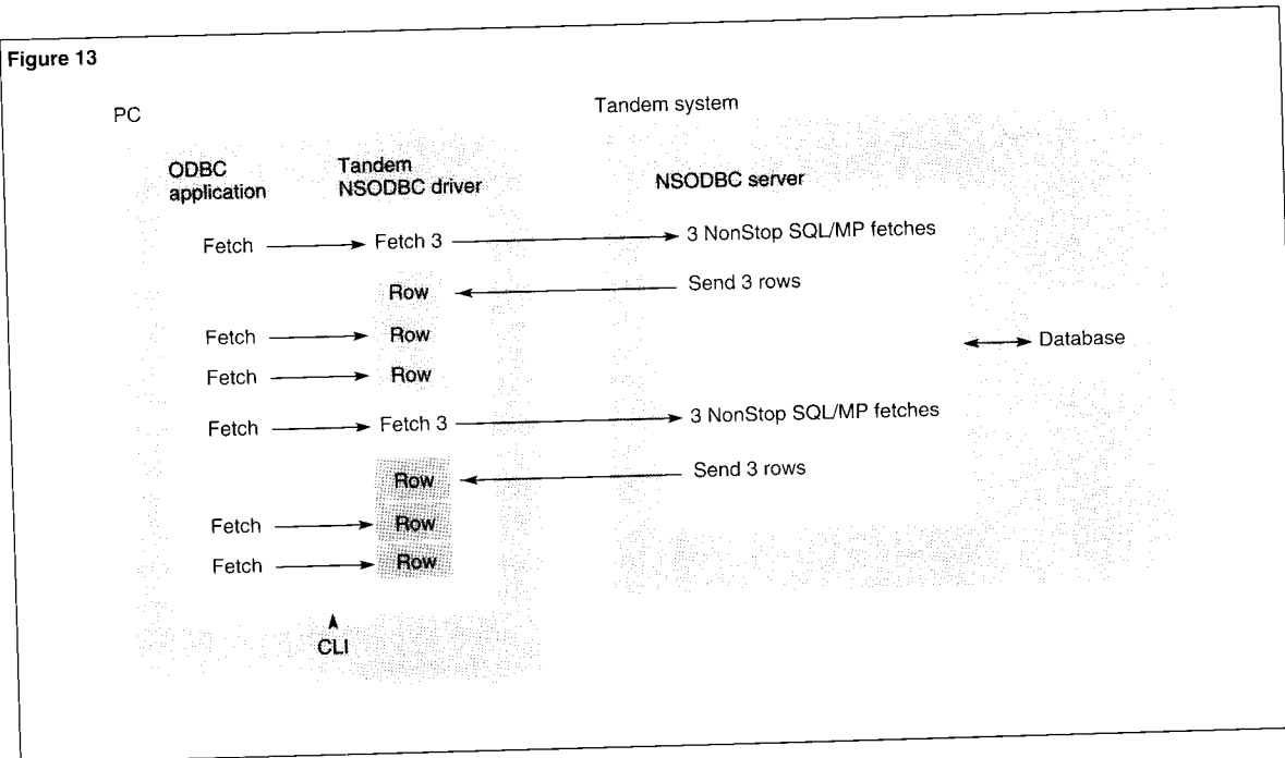
Figure 13. Bulk fetch for a core SQL client.
