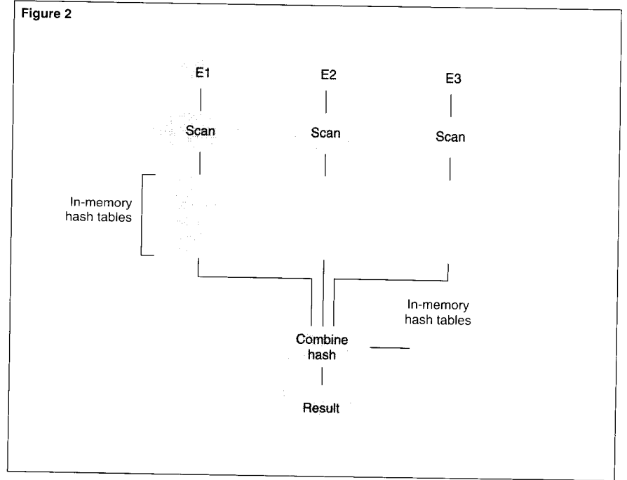
Figure 2. An example of a parallel hash grouping in NonStop SQL/MP.
