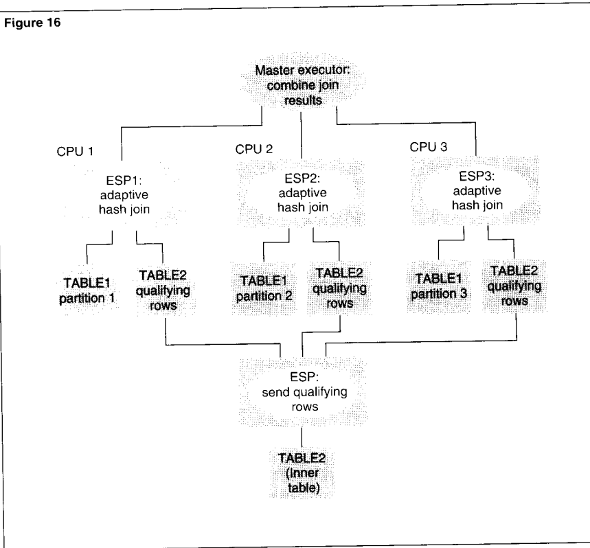
Figure 16. Parallel hash join on a partitioned table.
