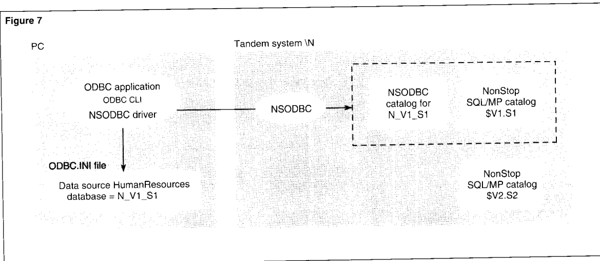
Figure 7. Access to a NonStop SQL/MP catalog requires an NSODBC catalog.
