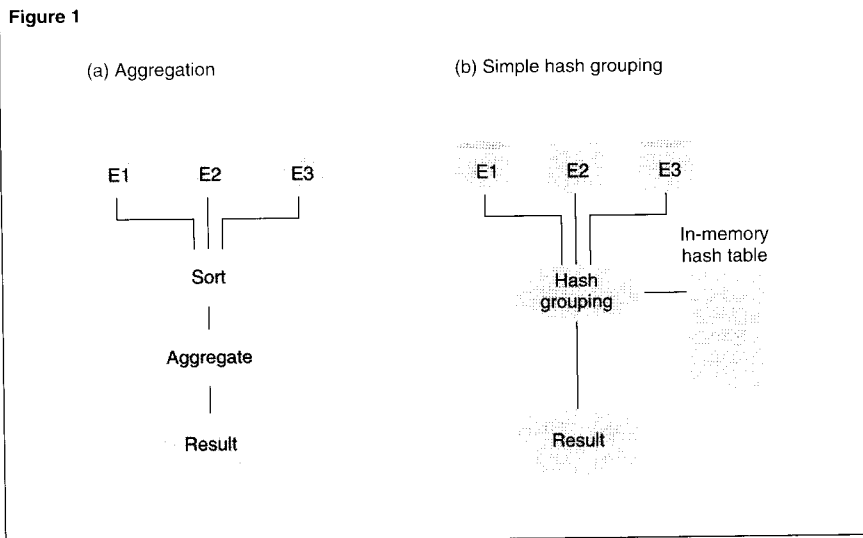
Figure 1. An example of a simple hash grouping. (a) Aggregation performed in previous releases of NonStop SQL. (b) Hash grouping performed by NonStop SQL/MP.
