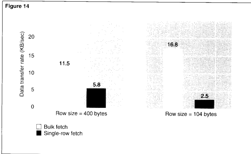
Figure 14. Comparison of data return rates for bulk fetch and single-row fetches.
