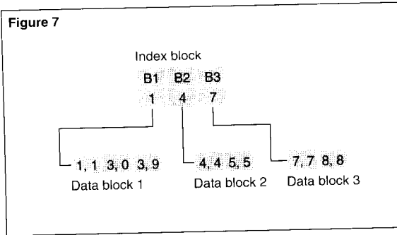
Figure 7. Partitioning of a table through B-tree indexing.
