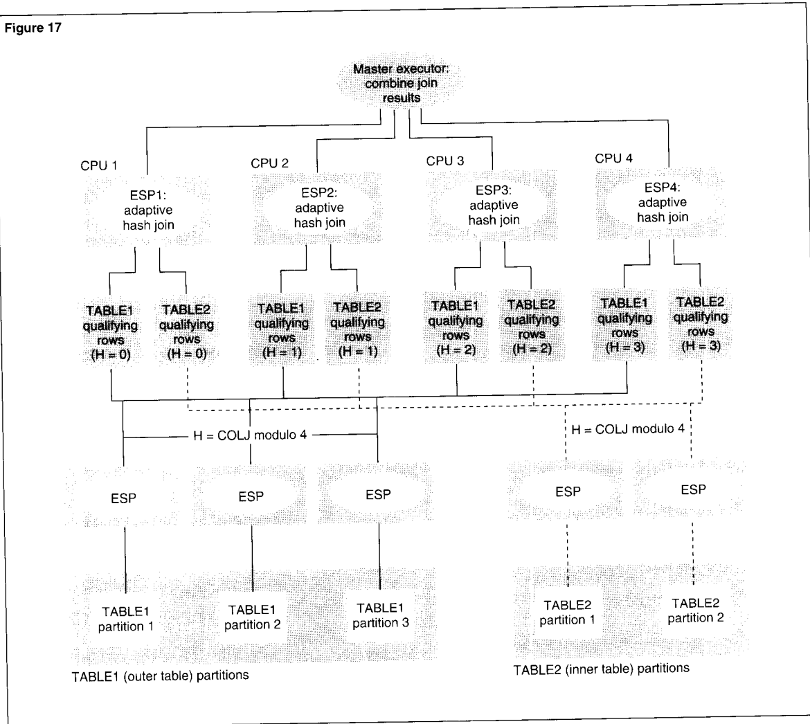
Figure 17. Hash-partitioned join with four CPUs.
