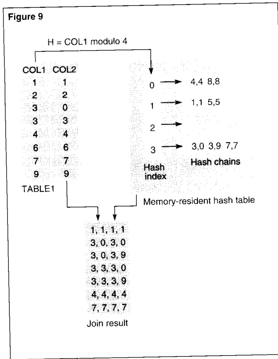
Figure 9. Probing phase of a hash join and join result.
