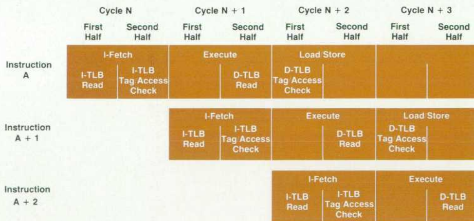
Fig. 6. TLB pipeline.
