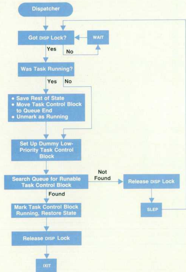
Fig. 2. Dispatcher flow chart.
