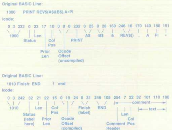
Fig. 3. Two examples of icode representations of BASIC program lines.
