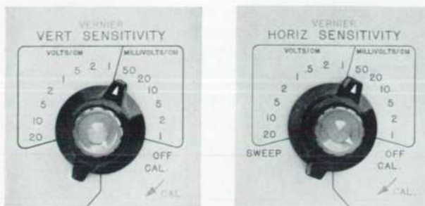
Fig. 8. Sensitivity of vertical and horizontal amplifiers is controlled by single, direct-reading switches. Sensitivity verniers are concentric with switch knob.
