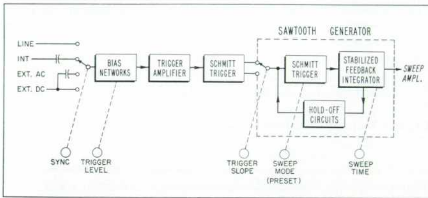
Fig. 3. Basic arrangement of trigger and sweep generator circuits. Use of triggered type sweep has many advantages as described in text.
