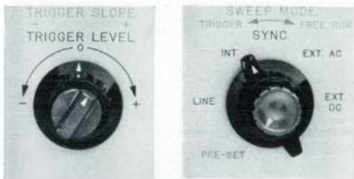
Fig. 5. Trigger controls on new hp-Model 130A . Concentric level- and slope-selecting controls are at left. Sync control at right selects source of trigger voltage. Sweep Mode adjusts sweep for free-running or triggered operation with Preset automatic triggering position at ccw end.
