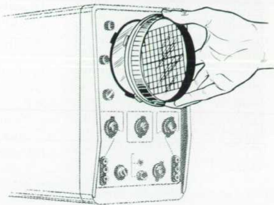
Fig. 13. Bezel can be removed or replaced by a 15° twist to facilitate filter or tube replacement.
