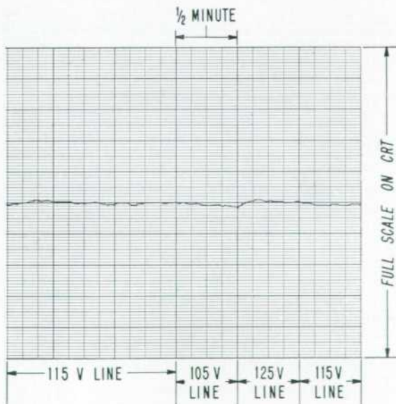
Fig. 10. Record of effect of line voltage changes on most sensitive range of oscilloscope. Height of chart is equal to full-scale deflection of oscilloscope.
