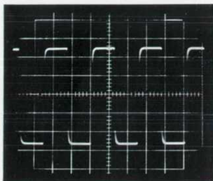
Fig. 9. Oscillogram of 40 kc square wave applied to vertical system. Sweep speed is 10 μsec/cm.
